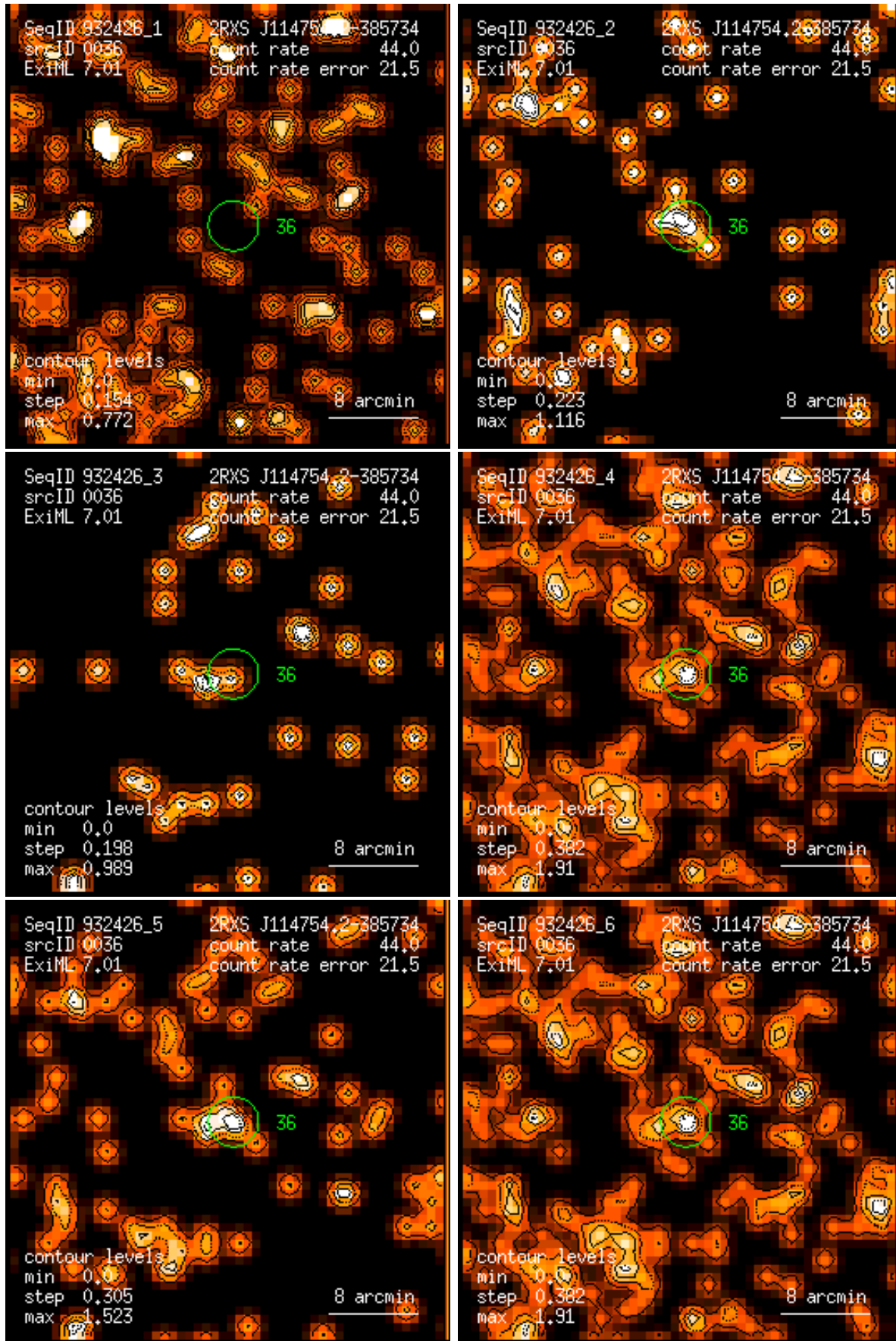
Figure 36: RASS 932426: detection 0036: band rate images, Gaussian filter: (1) PSPC channels 11 – 41, (2) 52 – 90, (3) 91 – 201, (4) 11 – 235, (5) 52 – 201, (6) 11 – 201. Broad band rates in counts/ks. Band rate contour levels in counts/ks/arcmin 2 .
