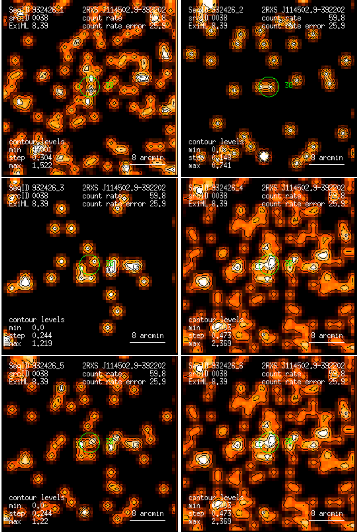
Figure 38: RASS 932426: detection 0038: band rate images, Gaussian filter: (1) PSPC channels 11 – 41, (2) 52 – 90, (3) 91 – 201, (4) 11 – 235, (5) 52 – 201, (6) 11 – 201. Broad band rates in counts/ks. Band rate contour levels in counts/ks/arcmin 2 .
