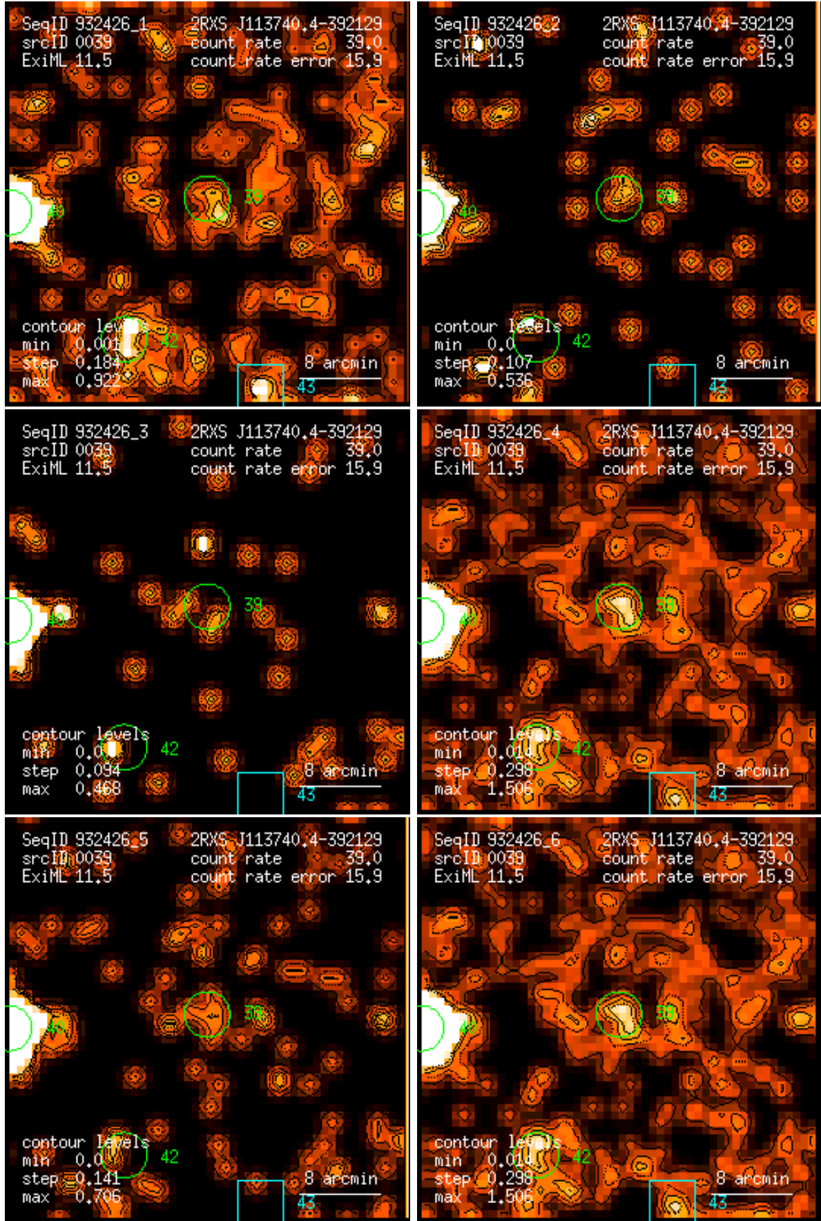
Figure 39: RASS 932426: detection 0039: band rate images, Gaussian filter: (1) PSPC channels 11 – 41, (2) 52 – 90, (3) 91 – 201, (4) 11 – 235, (5) 52 – 201, (6) 11 – 201. Broad band rates in counts/ks. Band rate contour levels in counts/ks/arcmin 2 .
