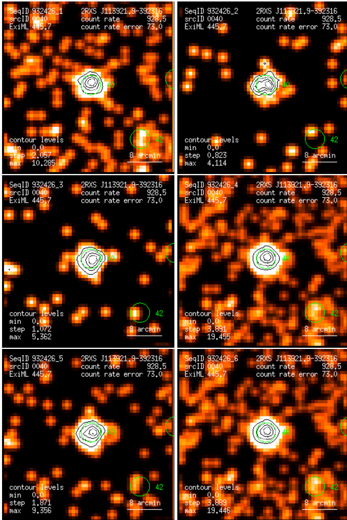
Figure 40: RASS 932426: detection 0040: band rate images, Gaussian filter: (1) PSPC channels 11 – 41, (2) 52 – 90, (3) 91 – 201, (4) 11 – 235, (5) 52 – 201, (6) 11 – 201. Broad band rates in counts/ks. Band rate contour levels in counts/ks/arcmin 2 .
