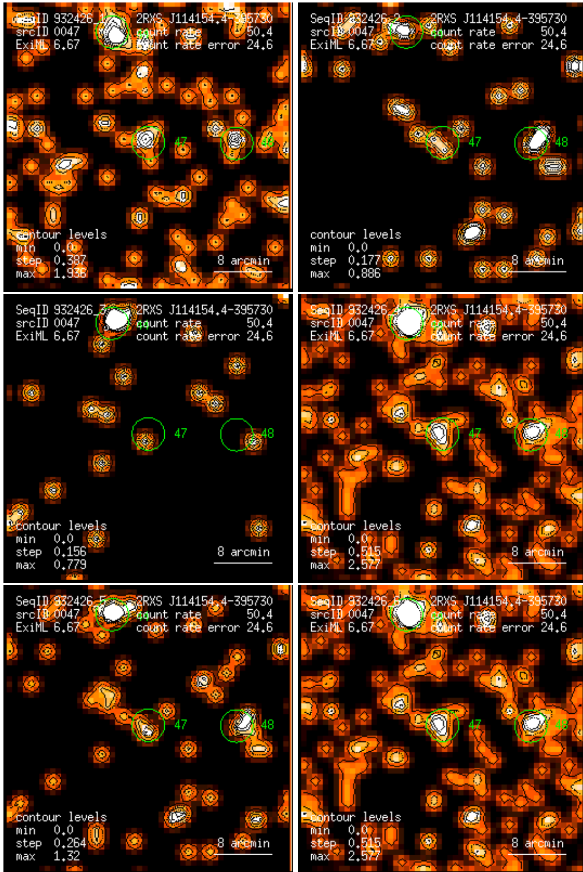
Figure 47: RASS 932426: detection 0047: band rate images, Gaussian filter: (1) PSPC channels 11 – 41, (2) 52 – 90, (3) 91 – 201, (4) 11 – 235, (5) 52 – 201, (6) 11 – 201. Broad band rates in counts/ks. Band rate contour levels in counts/ks/arcmin 2 .
