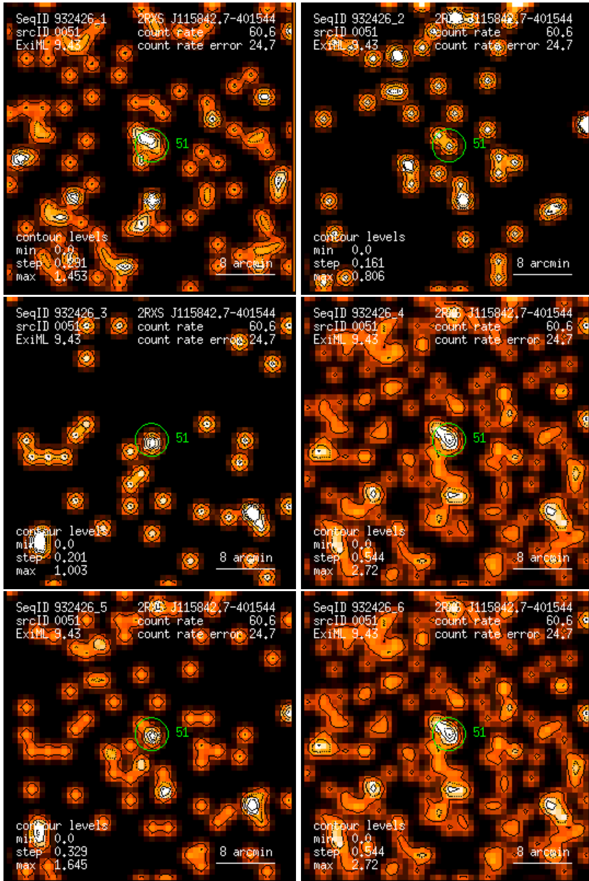
Figure 51: RASS 932426: detection 0051: band rate images, Gaussian filter: (1) PSPC channels 11 – 41, (2) 52 – 90, (3) 91 – 201, (4) 11 – 235, (5) 52 – 201, (6) 11 – 201. Broad band rates in counts/ks. Band rate contour levels in counts/ks/arcmin 2 .
