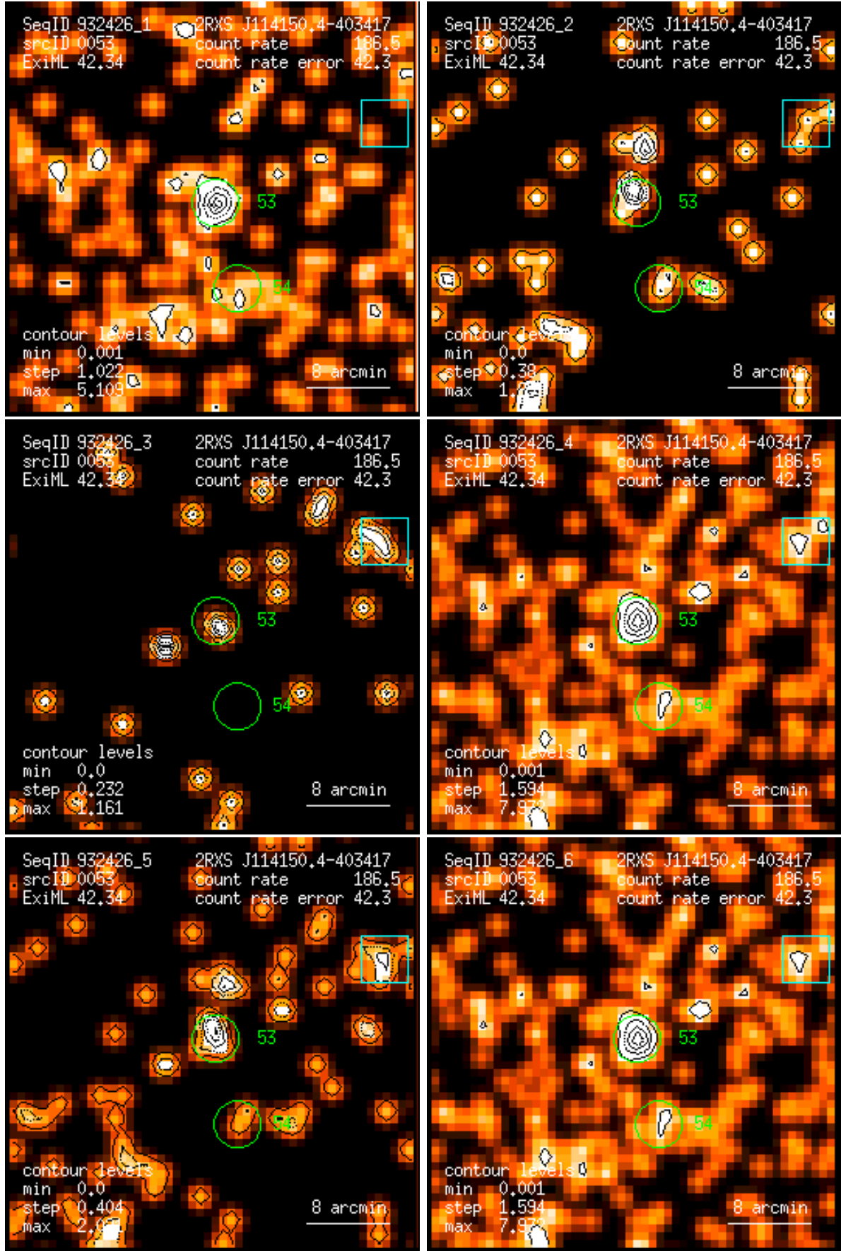
Figure 53: RASS 932426: detection 0053: band rate images, Gaussian filter: (1) PSPC channels 11 – 41, (2) 52 – 90, (3) 91 – 201, (4) 11 – 235, (5) 52 – 201, (6) 11 – 201. Broad band rates in counts/ks. Band rate contour levels in counts/ks/arcmin 2 .
