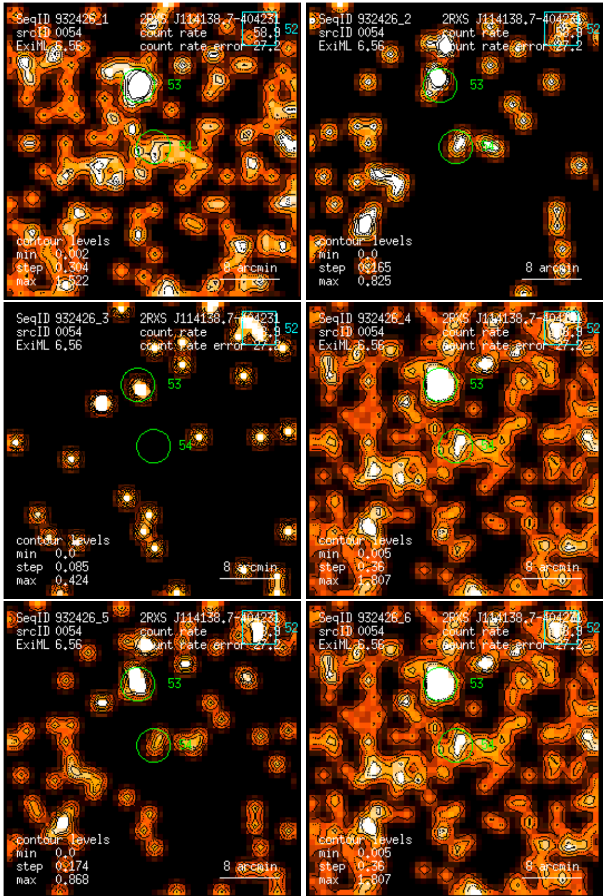
Figure 54: RASS 932426: detection 0054: band rate images, Gaussian filter: (1) PSPC channels 11 – 41, (2) 52 – 90, (3) 91 – 201, (4) 11 – 235, (5) 52 – 201, (6) 11 – 201. Broad band rates in counts/ks. Band rate contour levels in counts/ks/arcmin 2 .
