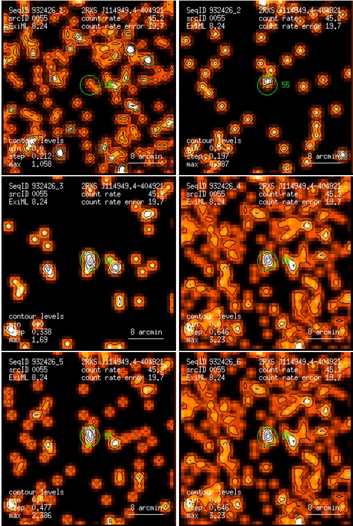
Figure 55: RASS 932426: detection 0055: band rate images, Gaussian filter: (1) PSPC channels 11 – 41, (2) 52 – 90, (3) 91 – 201, (4) 11 – 235, (5) 52 – 201, (6) 11 – 201. Broad band rates in counts/ks. Band rate contour levels in counts/ks/arcmin 2 .
