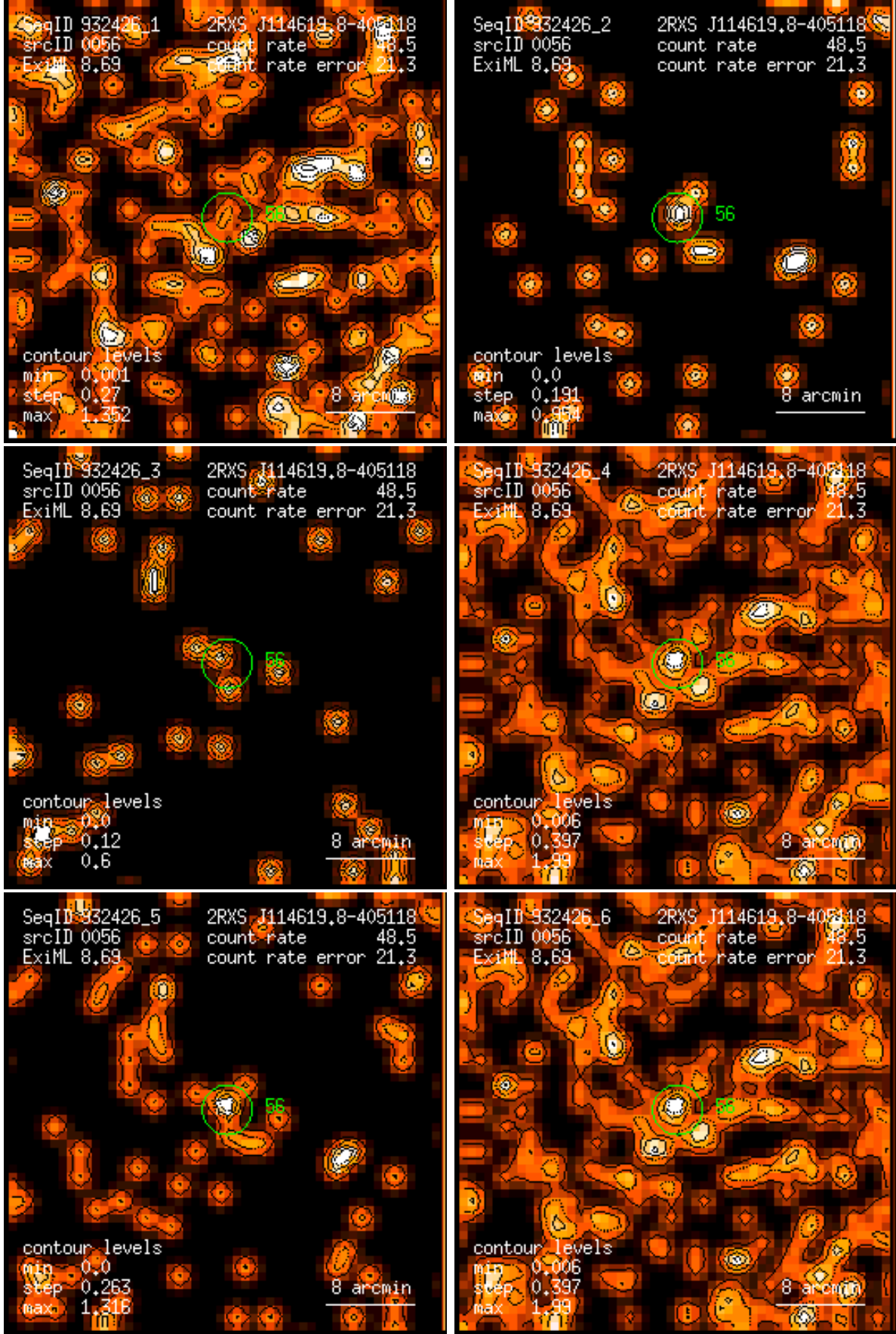
Figure 56: RASS 932426: detection 0056: band rate images, Gaussian filter: (1) PSPC channels 11 – 41, (2) 52 – 90, (3) 91 – 201, (4) 11 – 235, (5) 52 – 201, (6) 11 – 201. Broad band rates in counts/ks. Band rate contour levels in counts/ks/arcmin 2 .
