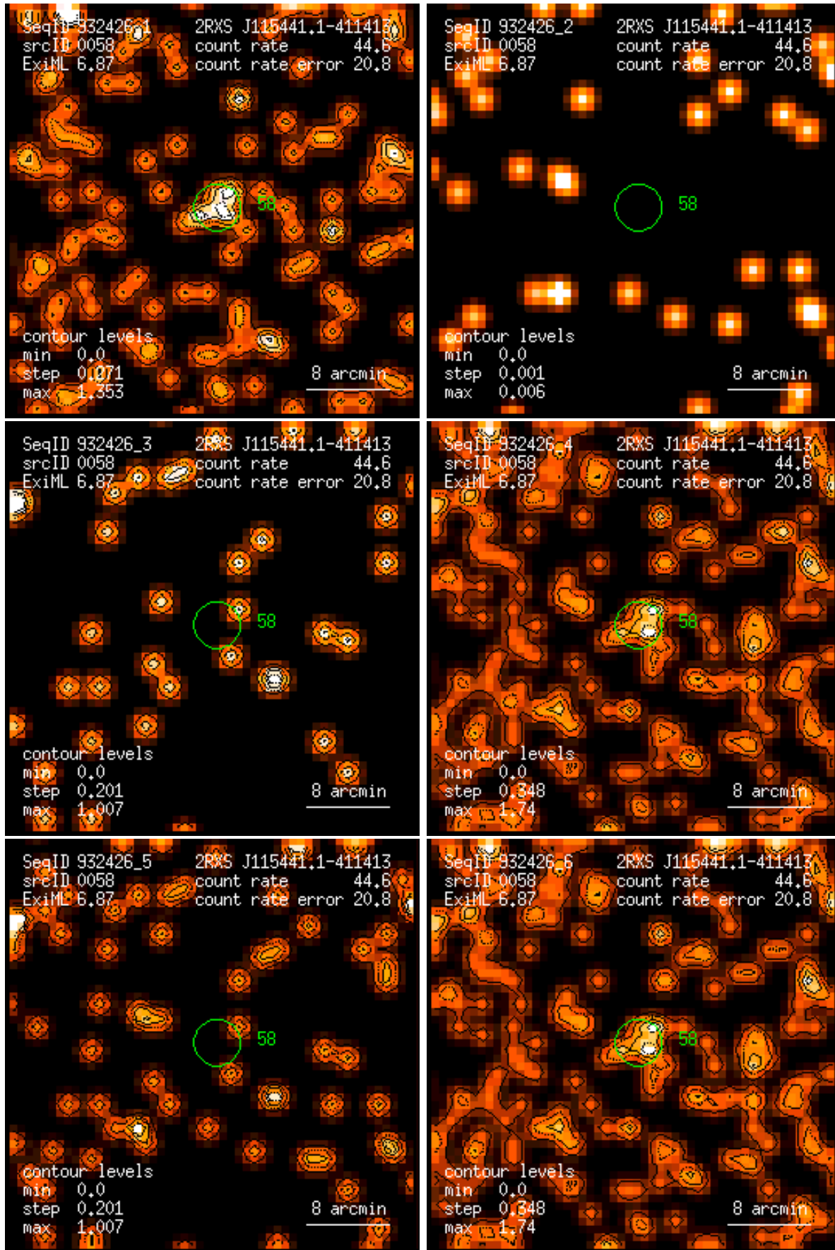
Figure 58: RASS 932426: detection 0058: band rate images, Gaussian filter: (1) PSPC channels 11 – 41, (2) 52 – 90, (3) 91 – 201, (4) 11 – 235, (5) 52 – 201, (6) 11 – 201. Broad band rates in counts/ks. Band rate contour levels in counts/ks/arcmin 2 .
