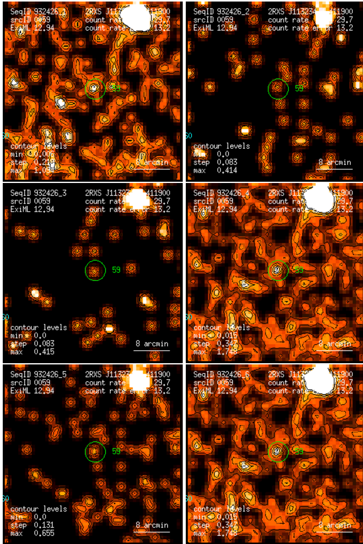
Figure 59: RASS 932426: detection 0059: band rate images, Gaussian filter: (1) PSPC channels 11 – 41, (2) 52 – 90, (3) 91 – 201, (4) 11 – 235, (5) 52 – 201, (6) 11 – 201. Broad band rates in counts/ks. Band rate contour levels in counts/ks/arcmin 2 .
