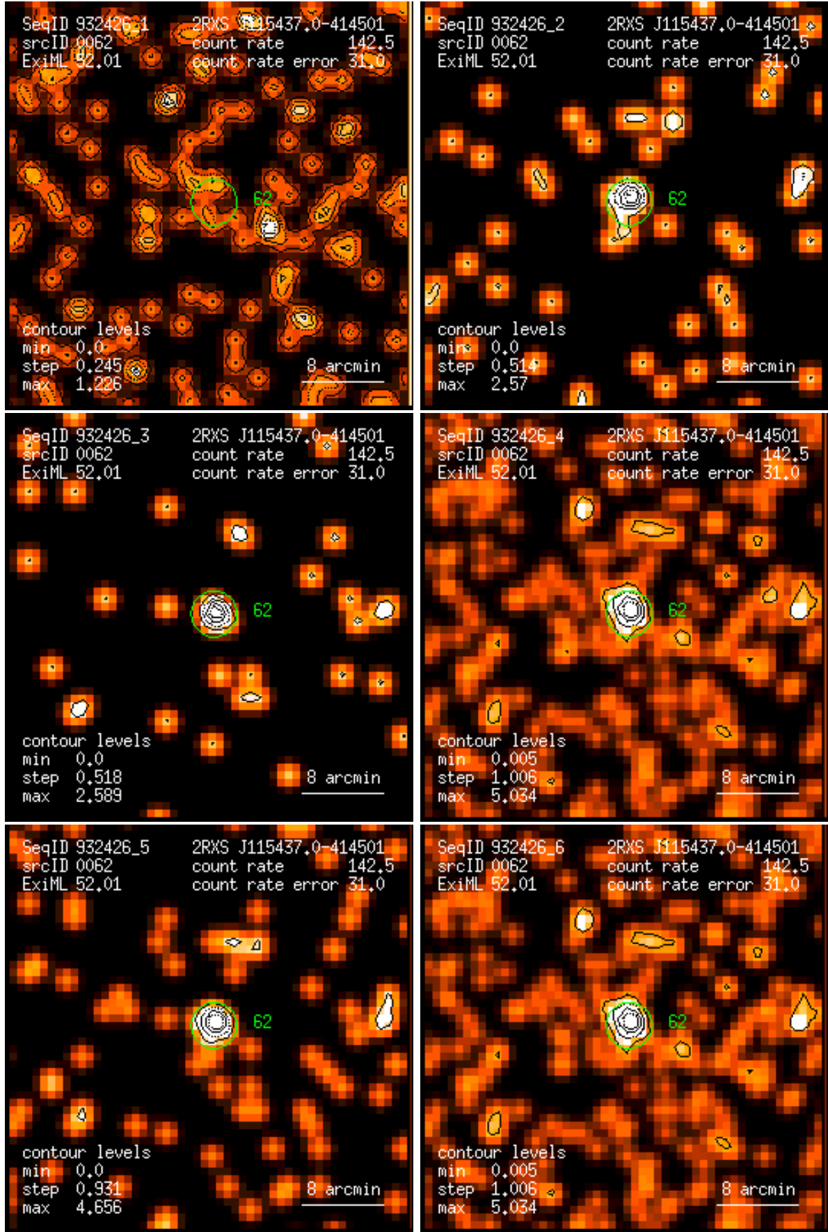
Figure 62: RASS 932426: detection 0062: band rate images, Gaussian filter: (1) PSPC channels 11 – 41, (2) 52 – 90, (3) 91 – 201, (4) 11 – 235, (5) 52 – 201, (6) 11 – 201. Broad band rates in counts/ks. Band rate contour levels in counts/ks/arcmin 2 .
