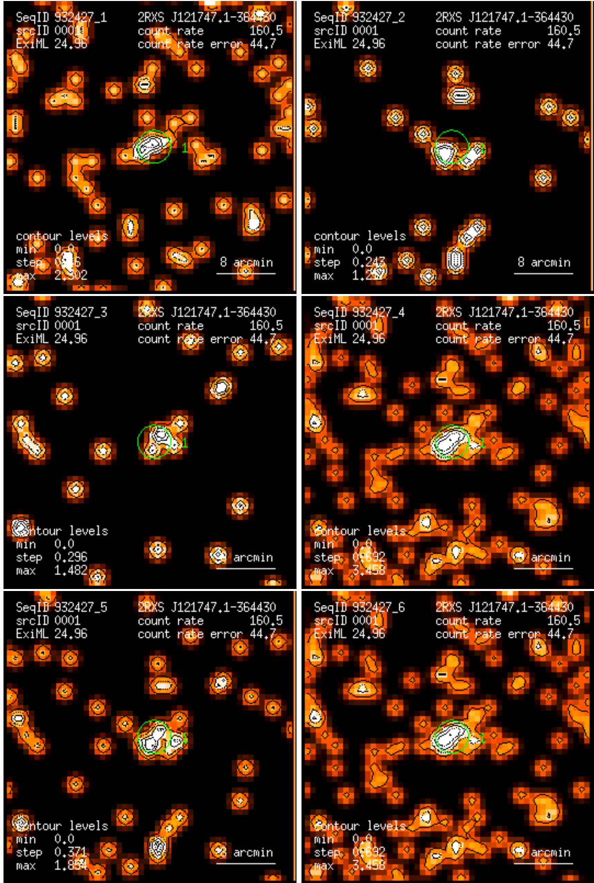
Figure 1: RASS 932427: detection 0001: band rate images, Gaussian filter: (1) PSPC channels 11 – 41, (2) 52 – 90, (3) 91 – 201, (4) 11 – 235, (5) 52 – 201, (6) 11 – 201. Broad band rates in counts/ks. Band rate contour levels in counts/ks/arcmin 2 .
