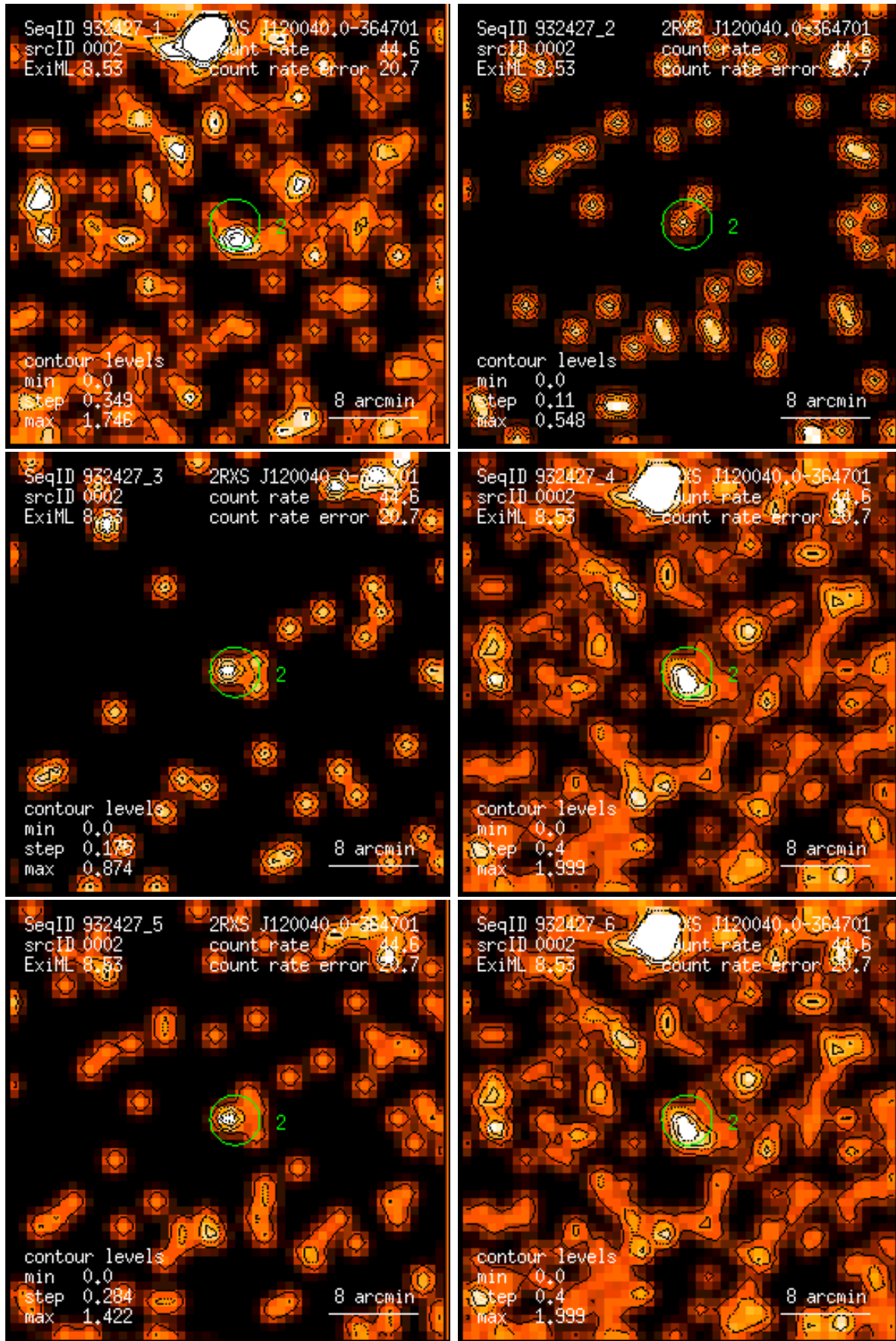
Figure 2: RASS 932427: detection 0002: band rate images, Gaussian filter: (1) PSPC channels 11 – 41, (2) 52 – 90, (3) 91 – 201, (4) 11 – 235, (5) 52 – 201, (6) 11 – 201. Broad band rates in counts/ks. Band rate contour levels in counts/ks/arcmin 2 .
