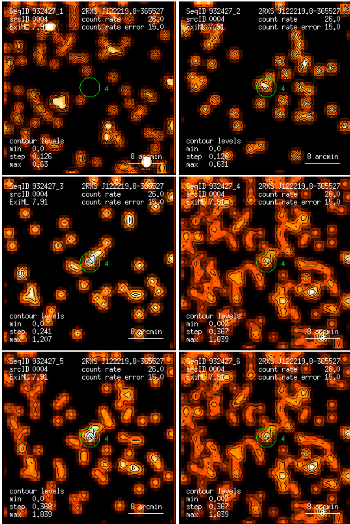
Figure 4: RASS 932427: detection 0004: band rate images, Gaussian filter: (1) PSPC channels 11 – 41, (2) 52 – 90, (3) 91 – 201, (4) 11 – 235, (5) 52 – 201, (6) 11 – 201. Broad band rates in counts/ks. Band rate contour levels in counts/ks/arcmin 2 .
