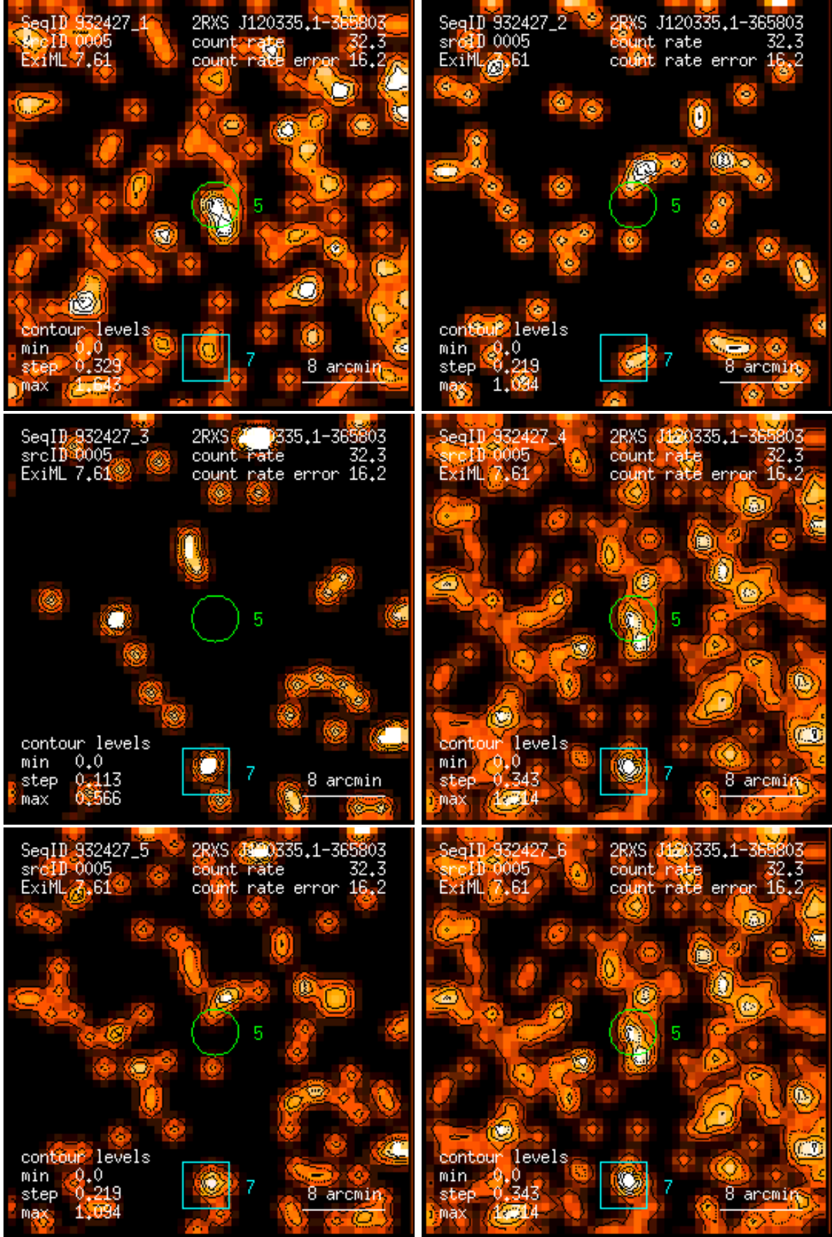
Figure 5: RASS 932427: detection 0005: band rate images, Gaussian filter: (1) PSPC channels 11 – 41, (2) 52 – 90, (3) 91 – 201, (4) 11 – 235, (5) 52 – 201, (6) 11 – 201. Broad band rates in counts/ks. Band rate contour levels in counts/ks/arcmin 2 .
