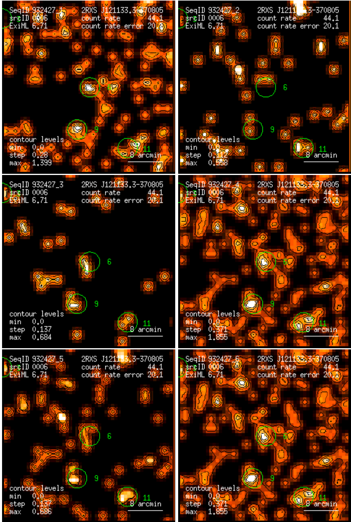
Figure 6: RASS 932427: detection 0006: band rate images, Gaussian filter: (1) PSPC channels 11 – 41, (2) 52 – 90, (3) 91 – 201, (4) 11 – 235, (5) 52 – 201, (6) 11 – 201. Broad band rates in counts/ks. Band rate contour levels in counts/ks/arcmin 2 .
