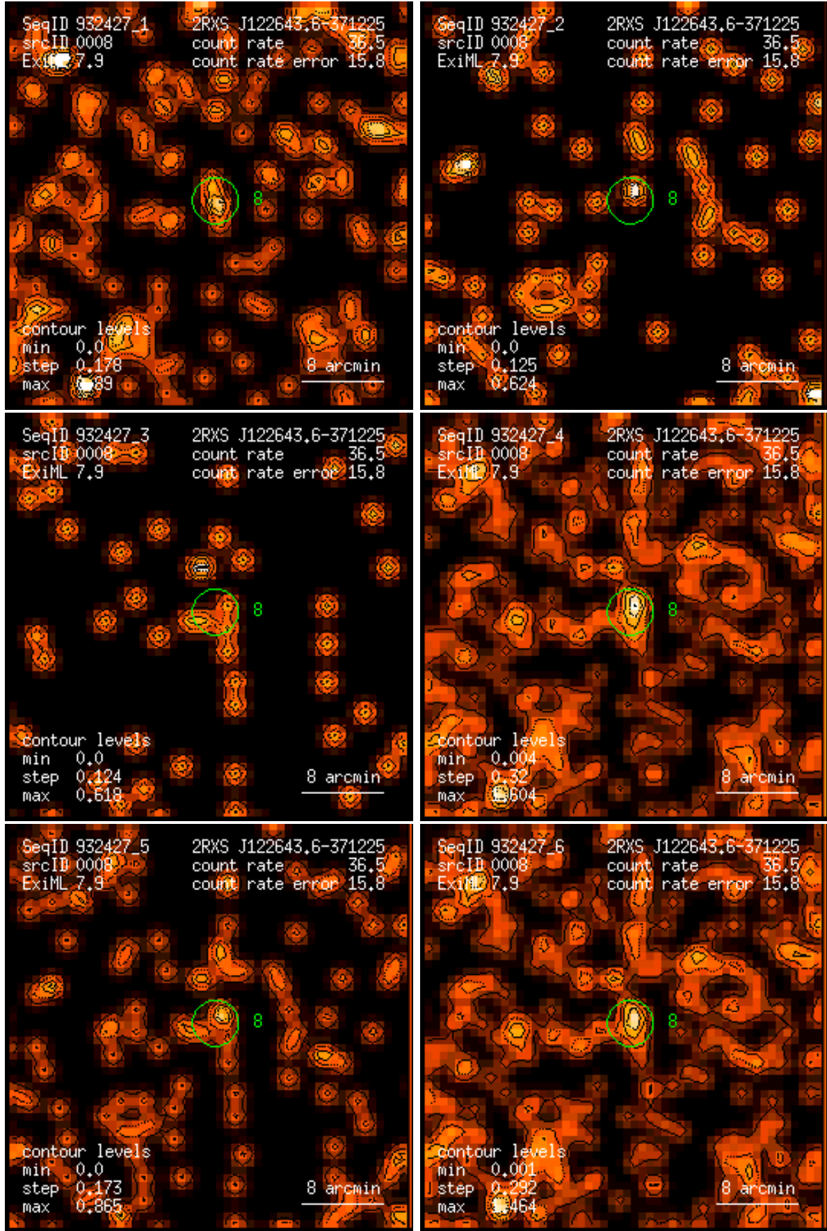
Figure 8: RASS 932427: detection 0008: band rate images, Gaussian filter: (1) PSPC channels 11 – 41, (2) 52 – 90, (3) 91 – 201, (4) 11 – 235, (5) 52 – 201, (6) 11 – 201. Broad band rates in counts/ks. Band rate contour levels in counts/ks/arcmin 2 .
