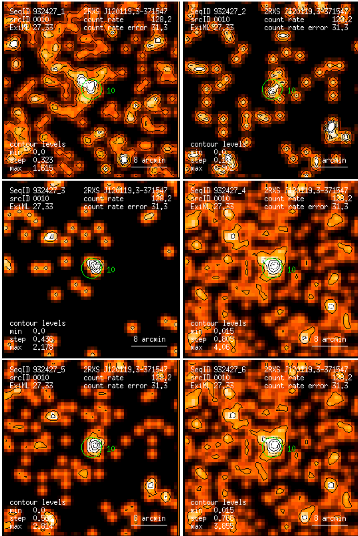
Figure 10: RASS 932427: detection 0010: band rate images, Gaussian filter: (1) PSPC channels 11 – 41, (2) 52 – 90, (3) 91 – 201, (4) 11 – 235, (5) 52 – 201, (6) 11 – 201. Broad band rates in counts/ks. Band rate contour levels in counts/ks/arcmin 2 .
