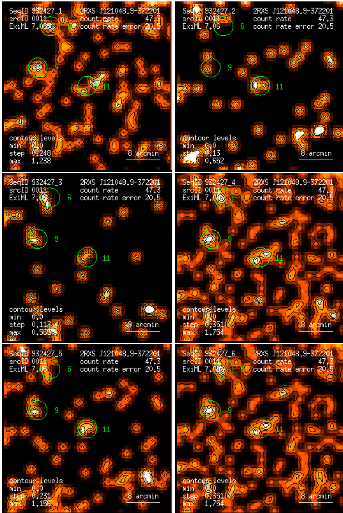
Figure 11: RASS 932427: detection 0011: band rate images, Gaussian filter: (1) PSPC channels 11 – 41, (2) 52 – 90, (3) 91 – 201, (4) 11 – 235, (5) 52 – 201, (6) 11 – 201. Broad band rates in counts/ks. Band rate contour levels in counts/ks/arcmin 2 .
