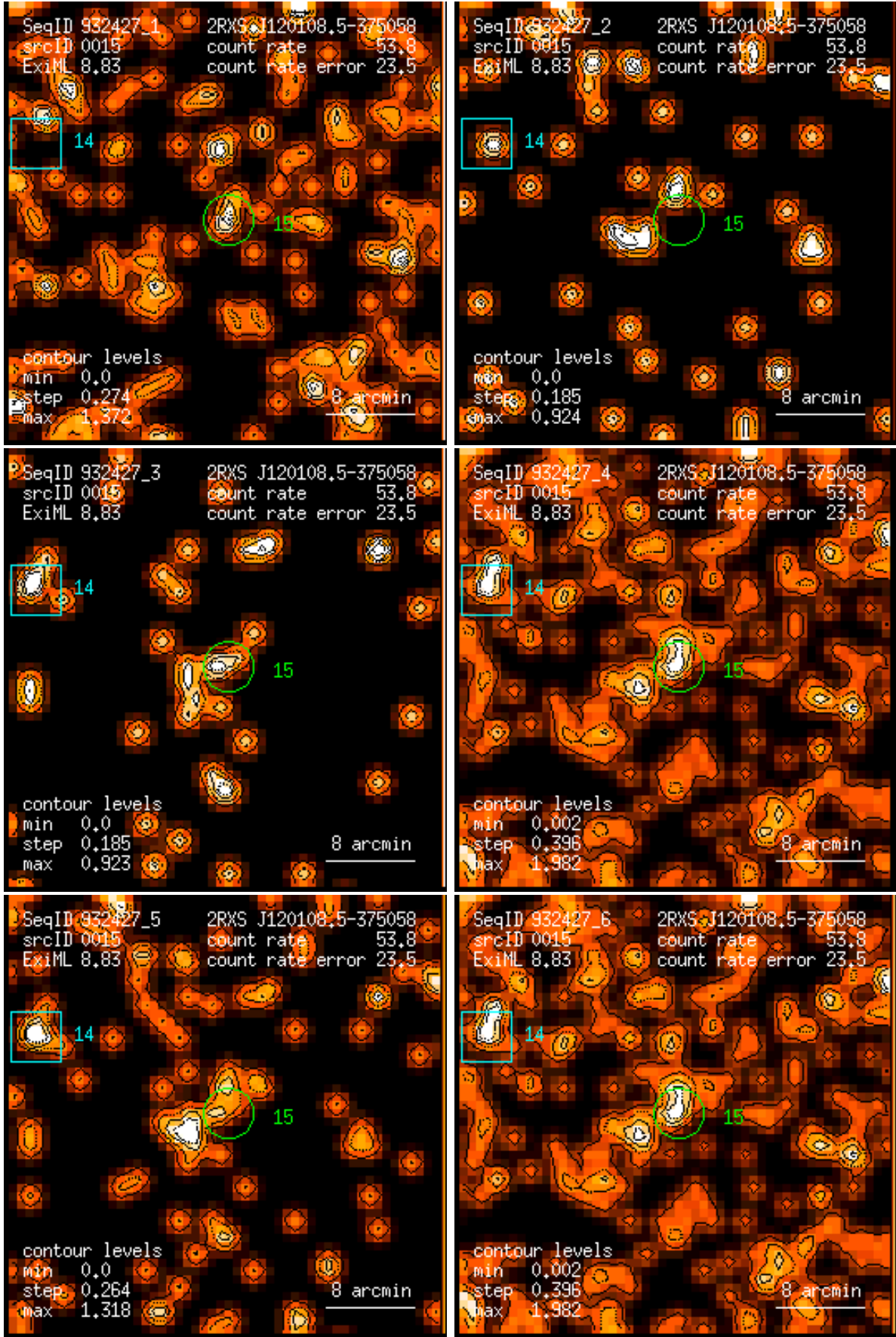
Figure 15: RASS 932427: detection 0015: band rate images, Gaussian filter: (1) PSPC channels 11 – 41, (2) 52 – 90, (3) 91 – 201, (4) 11 – 235, (5) 52 – 201, (6) 11 – 201. Broad band rates in counts/ks. Band rate contour levels in counts/ks/arcmin 2 .
