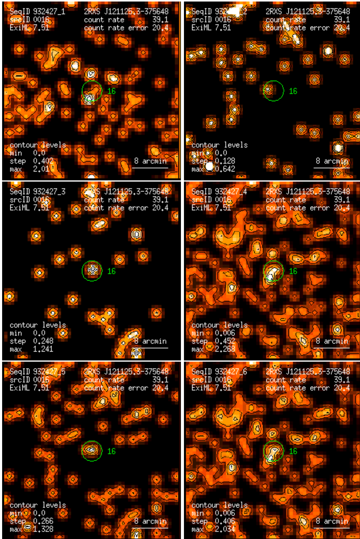
Figure 16: RASS 932427: detection 0016: band rate images, Gaussian filter: (1) PSPC channels 11 – 41, (2) 52 – 90, (3) 91 – 201, (4) 11 – 235, (5) 52 – 201, (6) 11 – 201. Broad band rates in counts/ks. Band rate contour levels in counts/ks/arcmin 2 .
