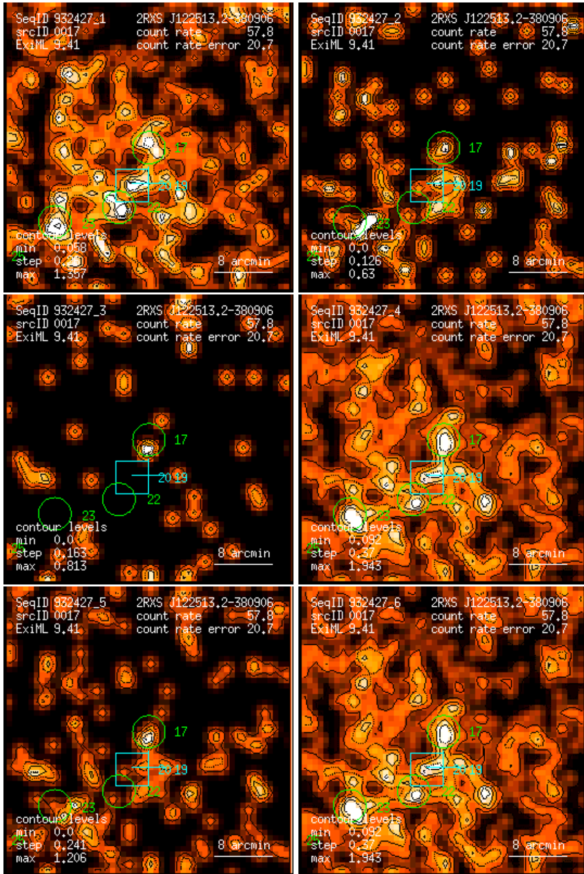
Figure 17: RASS 932427: detection 0017: band rate images, Gaussian filter: (1) PSPC channels 11 – 41, (2) 52 – 90, (3) 91 – 201, (4) 11 – 235, (5) 52 – 201, (6) 11 – 201. Broad band rates in counts/ks. Band rate contour levels in counts/ks/arcmin 2 .
