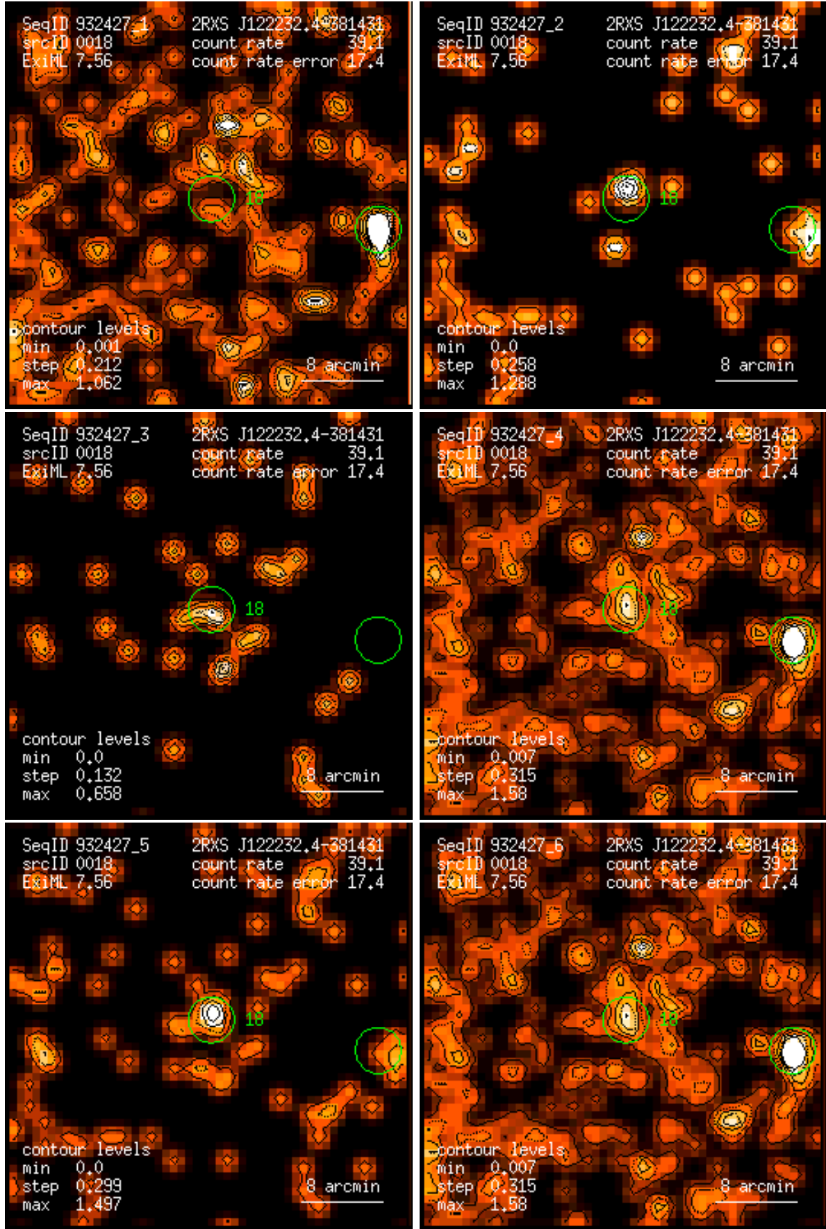
Figure 18: RASS 932427: detection 0018: band rate images, Gaussian filter: (1) PSPC channels 11 – 41, (2) 52 – 90, (3) 91 – 201, (4) 11 – 235, (5) 52 – 201, (6) 11 – 201. Broad band rates in counts/ks. Band rate contour levels in counts/ks/arcmin 2 .
