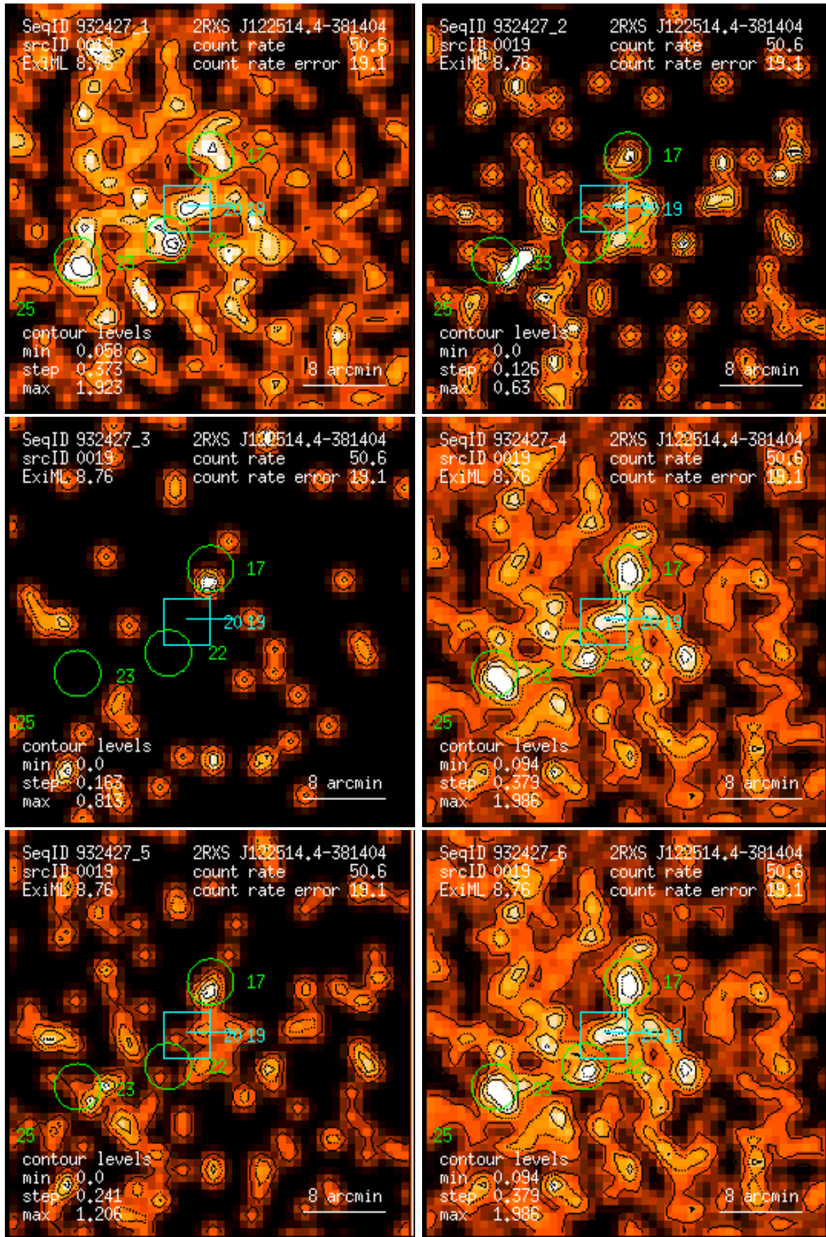
Figure 19: RASS 932427: detection 0019: band rate images, Gaussian filter: (1) PSPC channels 11 – 41, (2) 52 – 90, (3) 91 – 201, (4) 11 – 235, (5) 52 – 201, (6) 11 – 201. Broad band rates in counts/ks. Band rate contour levels in counts/ks/arcmin 2 .
