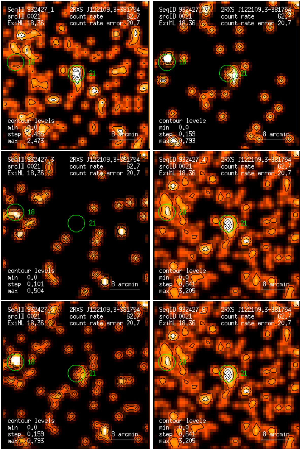
Figure 21: RASS 932427: detection 0021: band rate images, Gaussian filter: (1) PSPC channels 11 – 41, (2) 52 – 90, (3) 91 – 201, (4) 11 – 235, (5) 52 – 201, (6) 11 – 201. Broad band rates in counts/ks. Band rate contour levels in counts/ks/arcmin 2 .
