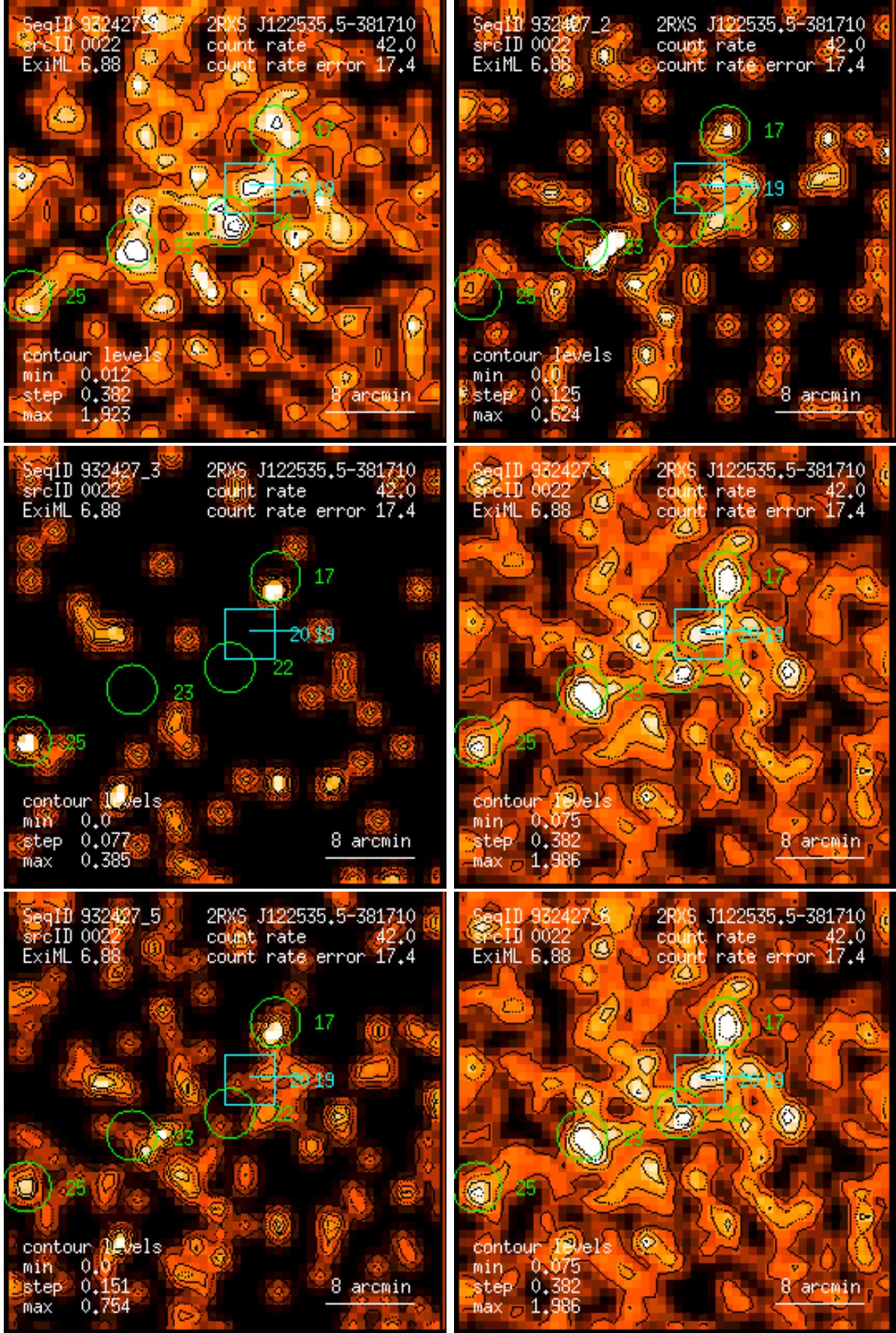
Figure 22: RASS 932427: detection 0022: band rate images, Gaussian filter: (1) PSPC channels 11 – 41, (2) 52 – 90, (3) 91 – 201, (4) 11 – 235, (5) 52 – 201, (6) 11 – 201. Broad band rates in counts/ks. Band rate contour levels in counts/ks/arcmin 2 .
