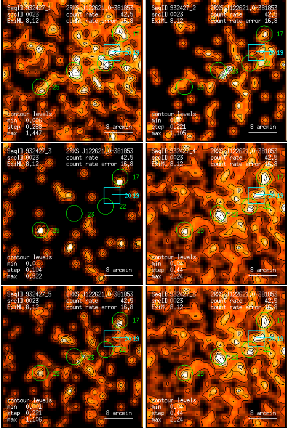
Figure 23: RASS 932427: detection 0023: band rate images, Gaussian filter: (1) PSPC channels 11 – 41, (2) 52 – 90, (3) 91 – 201, (4) 11 – 235, (5) 52 – 201, (6) 11 – 201. Broad band rates in counts/ks. Band rate contour levels in counts/ks/arcmin 2 .
