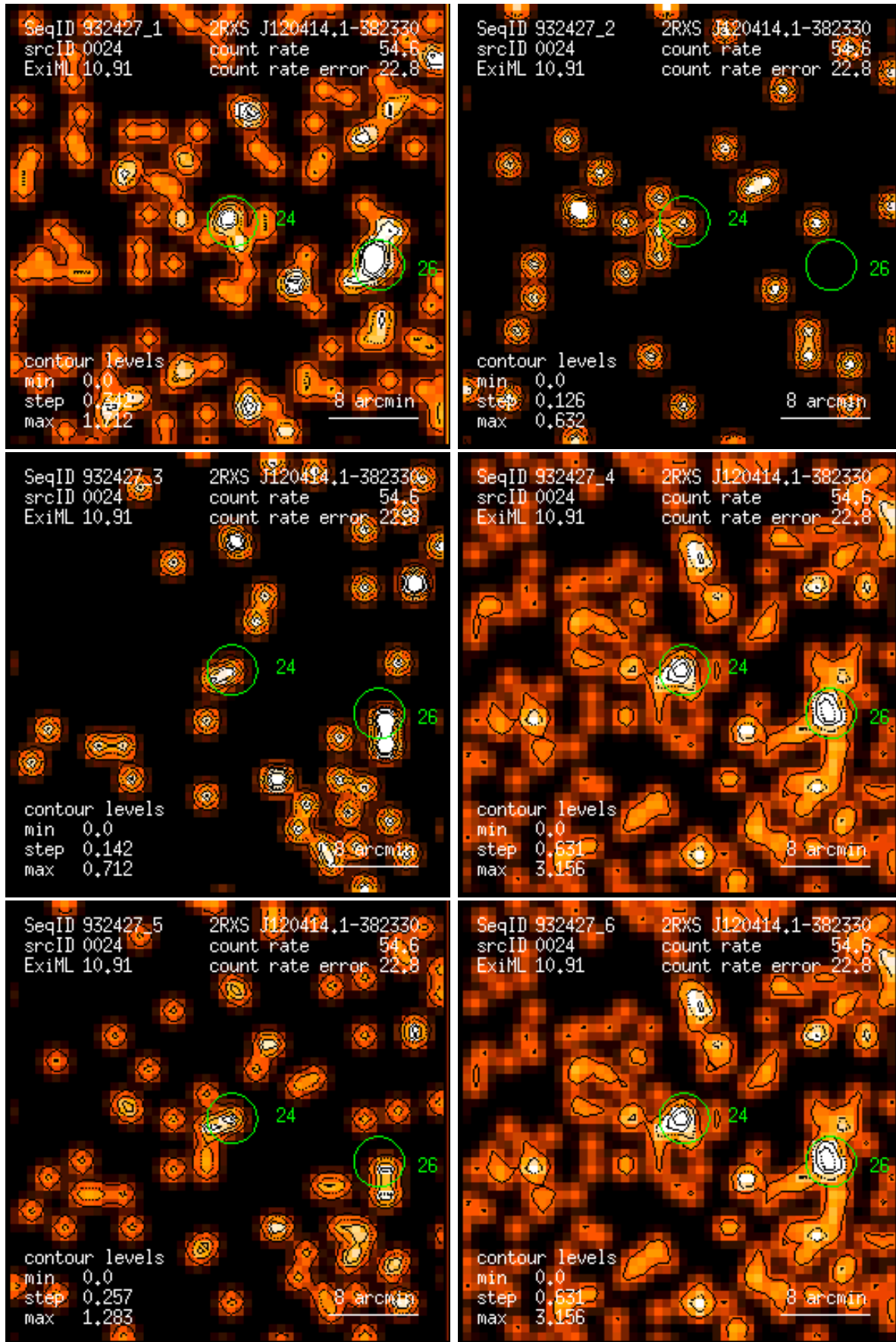
Figure 24: RASS 932427: detection 0024: band rate images, Gaussian filter: (1) PSPC channels 11 – 41, (2) 52 – 90, (3) 91 – 201, (4) 11 – 235, (5) 52 – 201, (6) 11 – 201. Broad band rates in counts/ks. Band rate contour levels in counts/ks/arcmin 2 .
