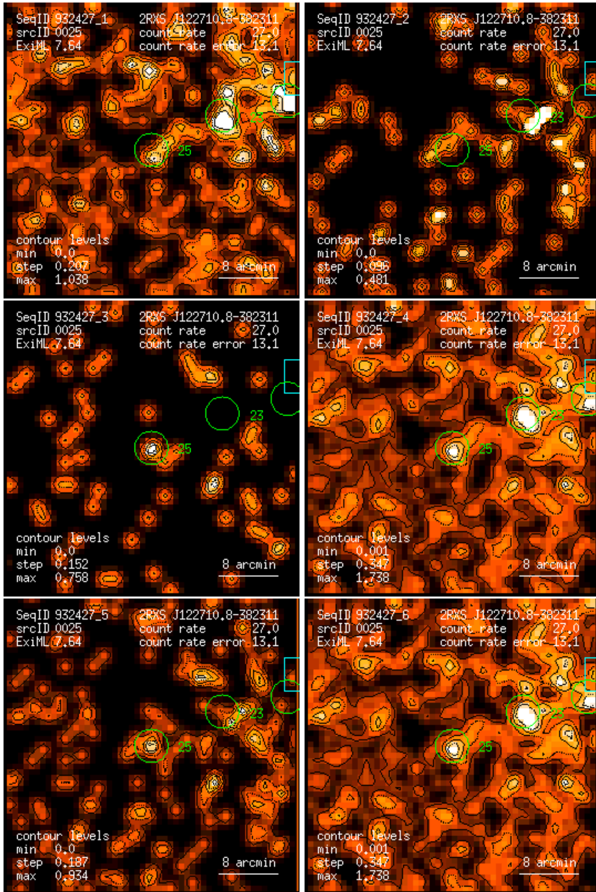
Figure 25: RASS 932427: detection 0025: band rate images, Gaussian filter: (1) PSPC channels 11 – 41, (2) 52 – 90, (3) 91 – 201, (4) 11 – 235, (5) 52 – 201, (6) 11 – 201. Broad band rates in counts/ks. Band rate contour levels in counts/ks/arcmin 2 .
