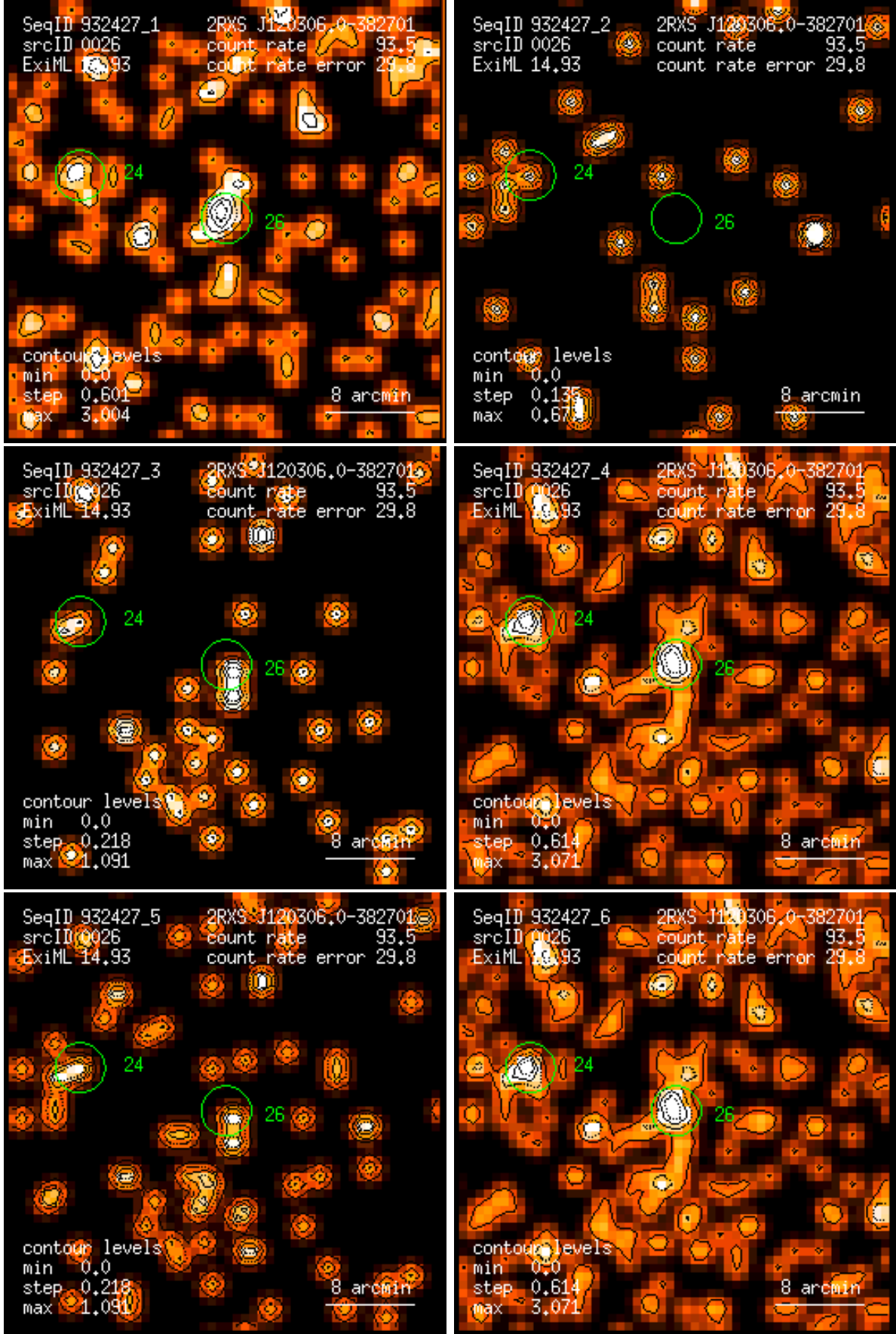
Figure 26: RASS 932427: detection 0026: band rate images, Gaussian filter: (1) PSPC channels 11 – 41, (2) 52 – 90, (3) 91 – 201, (4) 11 – 235, (5) 52 – 201, (6) 11 – 201. Broad band rates in counts/ks. Band rate contour levels in counts/ks/arcmin 2 .
