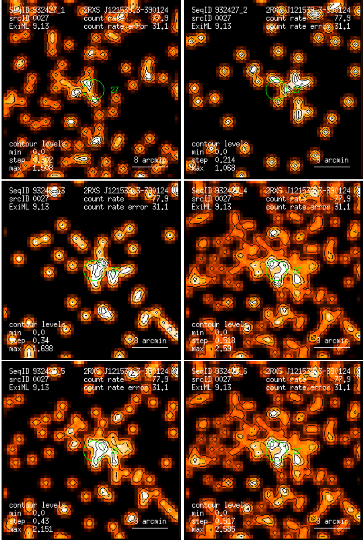
Figure 27: RASS 932427: detection 0027: band rate images, Gaussian filter: (1) PSPC channels 11 – 41, (2) 52 – 90, (3) 91 – 201, (4) 11 – 235, (5) 52 – 201, (6) 11 – 201. Broad band rates in counts/ks. Band rate contour levels in counts/ks/arcmin 2 .
