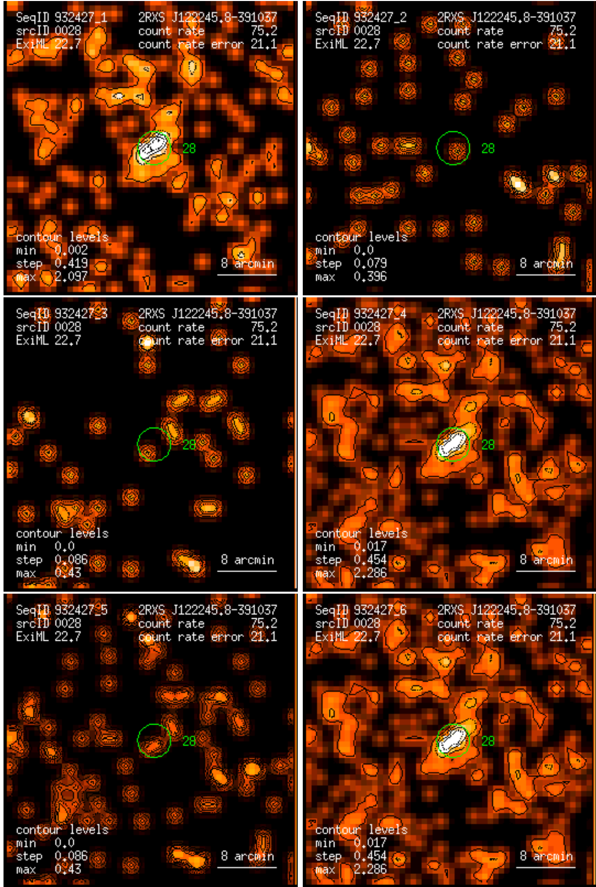
Figure 28: RASS 932427: detection 0028: band rate images, Gaussian filter: (1) PSPC channels 11 – 41, (2) 52 – 90, (3) 91 – 201, (4) 11 – 235, (5) 52 – 201, (6) 11 – 201. Broad band rates in counts/ks. Band rate contour levels in counts/ks/arcmin 2 .
