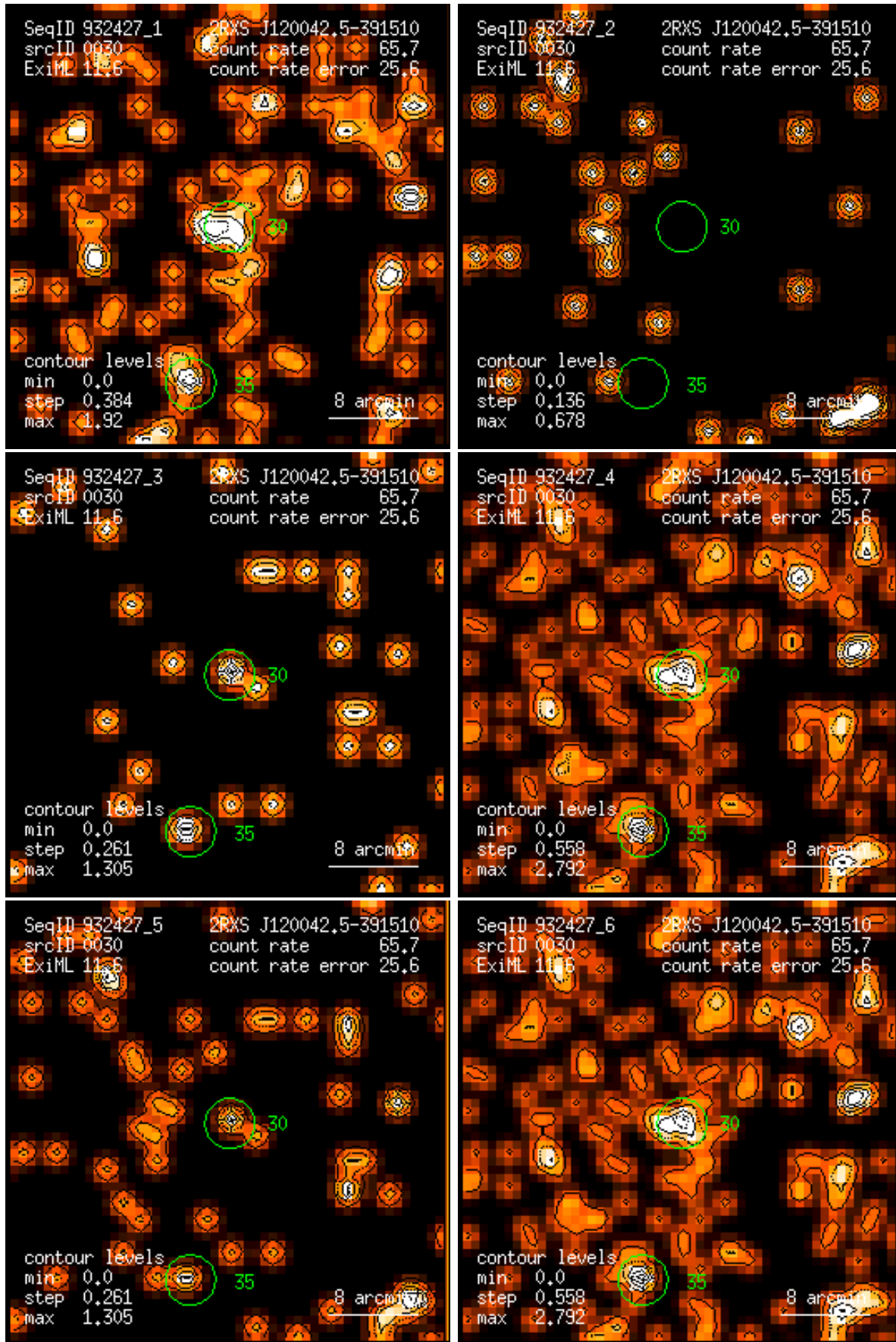
Figure 30: RASS 932427: detection 0030: band rate images, Gaussian filter: (1) PSPC channels 11 – 41, (2) 52 – 90, (3) 91 – 201, (4) 11 – 235, (5) 52 – 201, (6) 11 – 201. Broad band rates in counts/ks. Band rate contour levels in counts/ks/arcmin 2 .
