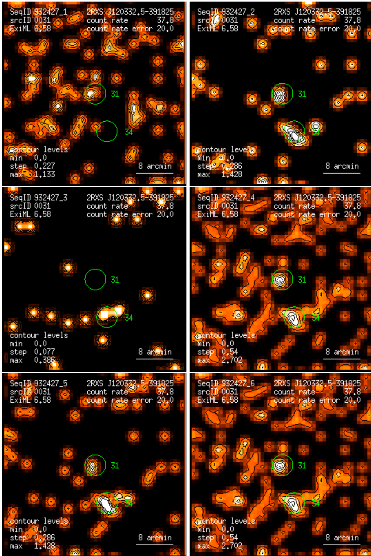
Figure 31: RASS 932427: detection 0031: band rate images, Gaussian filter: (1) PSPC channels 11 – 41, (2) 52 – 90, (3) 91 – 201, (4) 11 – 235, (5) 52 – 201, (6) 11 – 201. Broad band rates in counts/ks. Band rate contour levels in counts/ks/arcmin 2 .
