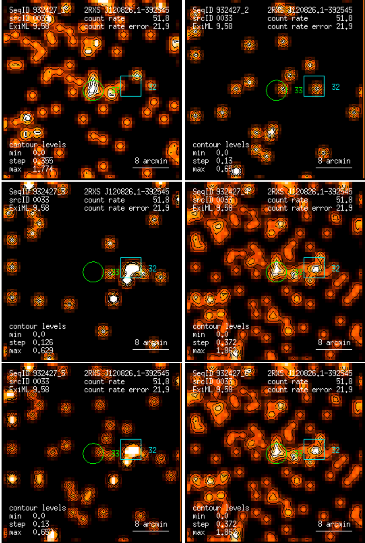
Figure 33: RASS 932427: detection 0033: band rate images, Gaussian filter: (1) PSPC channels 11 – 41, (2) 52 – 90, (3) 91 – 201, (4) 11 – 235, (5) 52 – 201, (6) 11 – 201. Broad band rates in counts/ks. Band rate contour levels in counts/ks/arcmin 2 .
