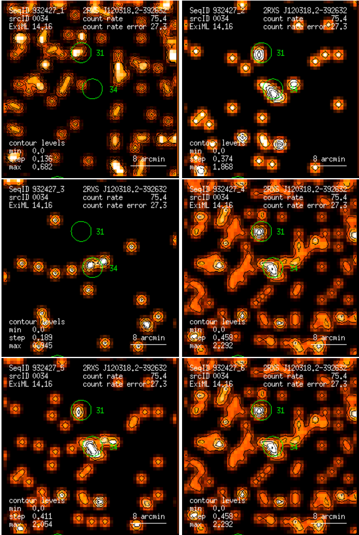
Figure 34: RASS 932427: detection 0034: band rate images, Gaussian filter: (1) PSPC channels 11 – 41, (2) 52 – 90, (3) 91 – 201, (4) 11 – 235, (5) 52 – 201, (6) 11 – 201. Broad band rates in counts/ks. Band rate contour levels in counts/ks/arcmin 2 .
