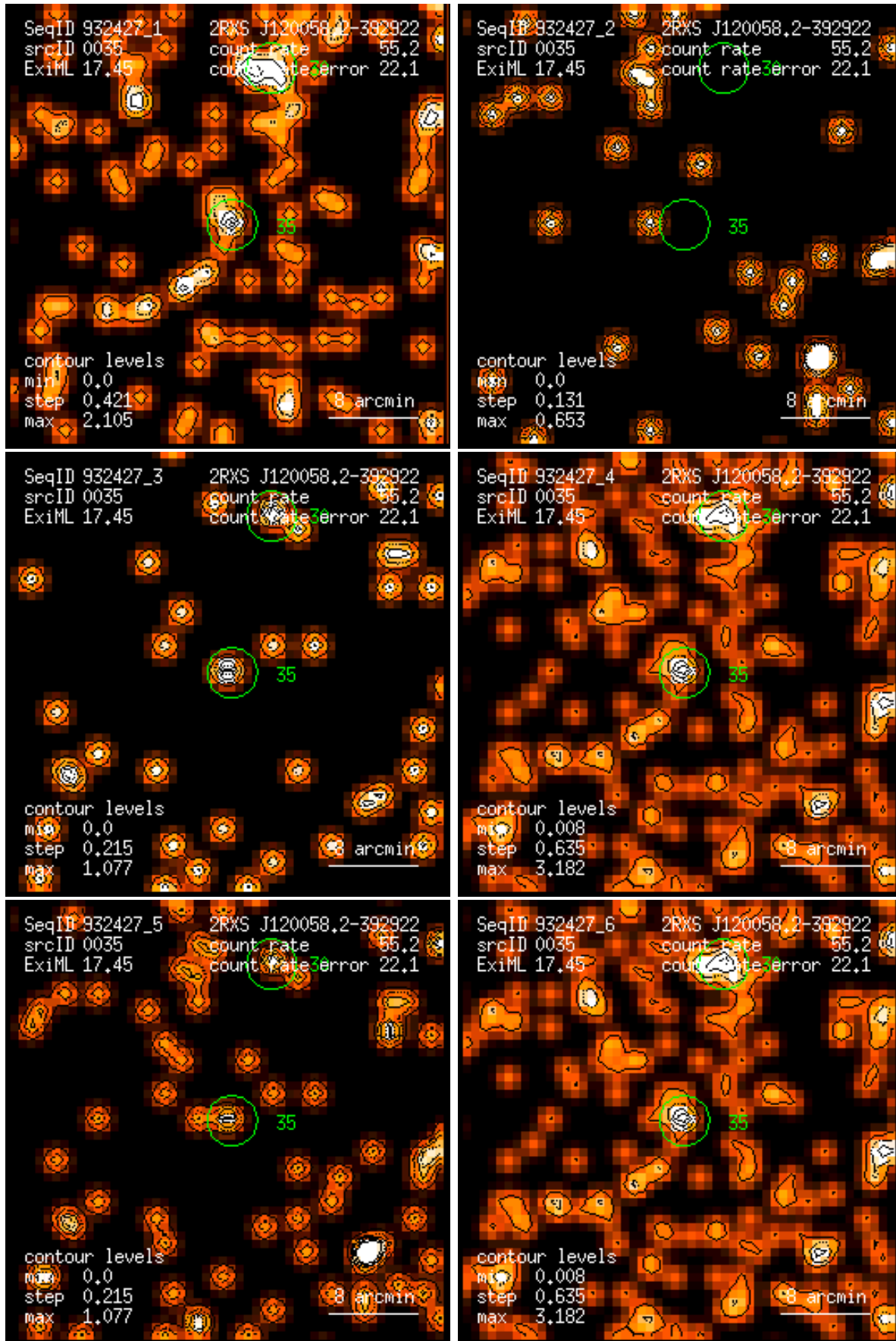
Figure 35: RASS 932427: detection 0035: band rate images, Gaussian filter: (1) PSPC channels 11 – 41, (2) 52 – 90, (3) 91 – 201, (4) 11 – 235, (5) 52 – 201, (6) 11 – 201. Broad band rates in counts/ks. Band rate contour levels in counts/ks/arcmin 2 .
