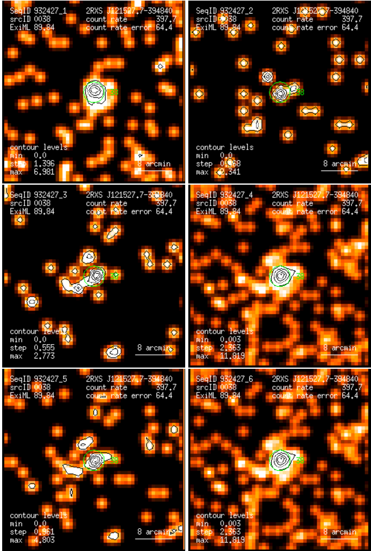
Figure 38: RASS 932427: detection 0038: band rate images, Gaussian filter: (1) PSPC channels 11 – 41, (2) 52 – 90, (3) 91 – 201, (4) 11 – 235, (5) 52 – 201, (6) 11 – 201. Broad band rates in counts/ks. Band rate contour levels in counts/ks/arcmin 2 .
