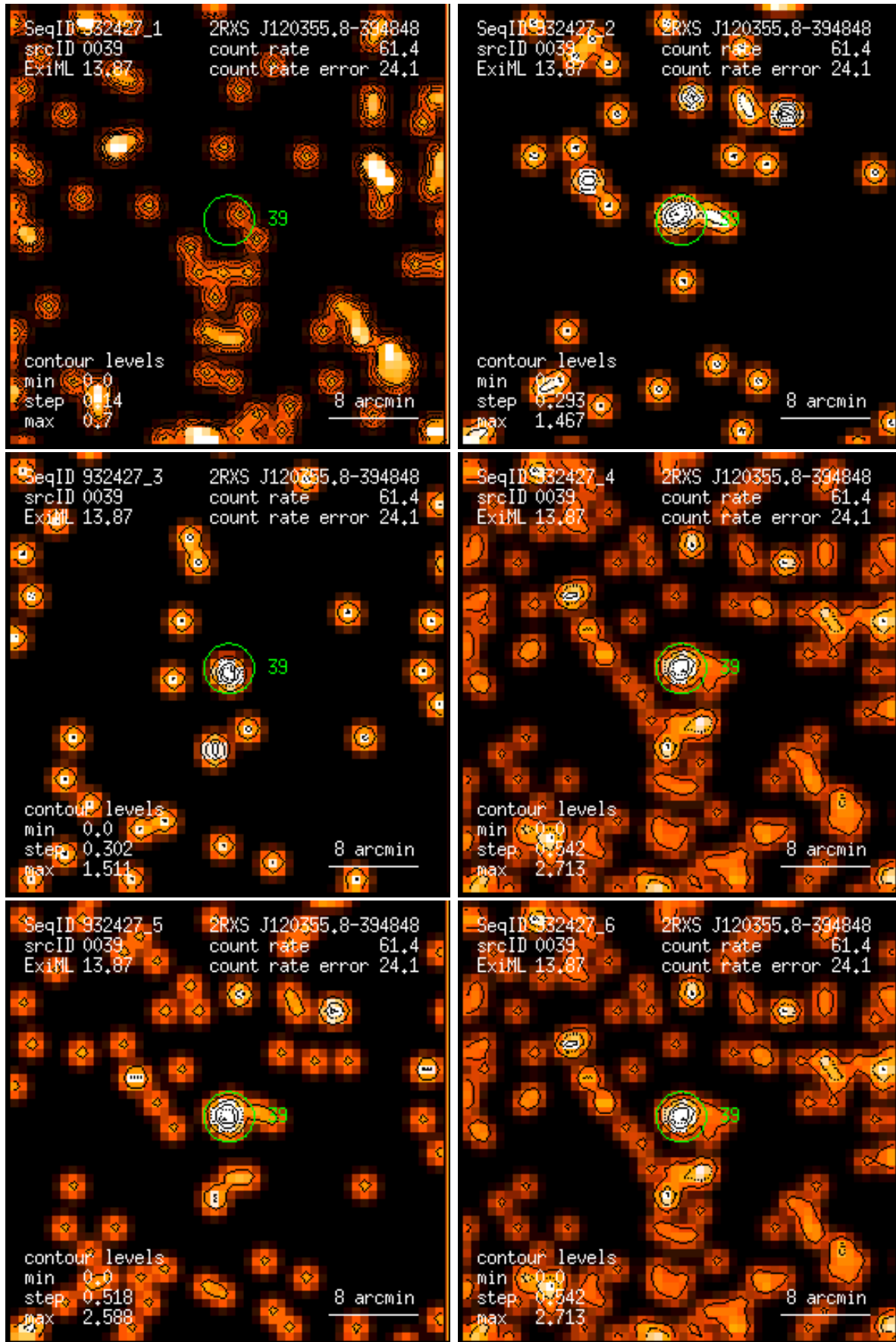
Figure 39: RASS 932427: detection 0039: band rate images, Gaussian filter: (1) PSPC channels 11 – 41, (2) 52 – 90, (3) 91 – 201, (4) 11 – 235, (5) 52 – 201, (6) 11 – 201. Broad band rates in counts/ks. Band rate contour levels in counts/ks/arcmin 2 .
