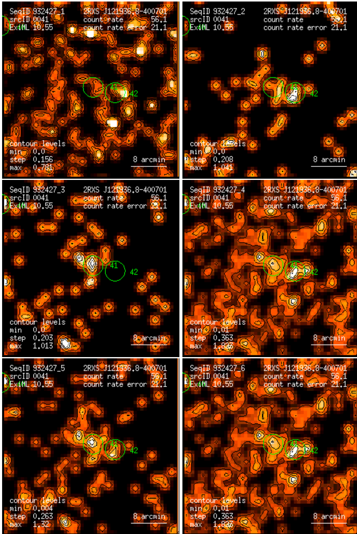
Figure 41: RASS 932427: detection 0041: band rate images, Gaussian filter: (1) PSPC channels 11 – 41, (2) 52 – 90, (3) 91 – 201, (4) 11 – 235, (5) 52 – 201, (6) 11 – 201. Broad band rates in counts/ks. Band rate contour levels in counts/ks/arcmin 2 .
