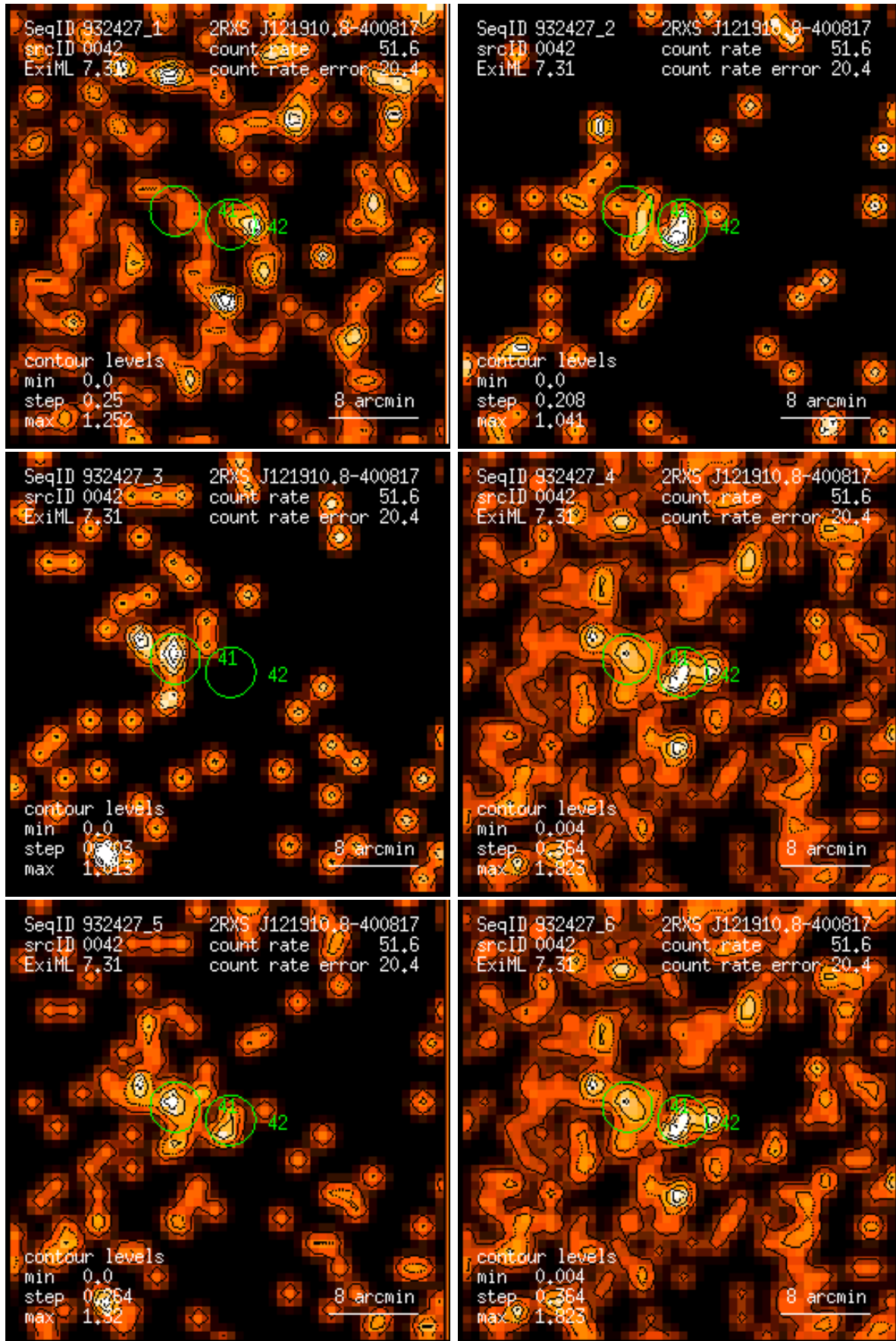
Figure 42: RASS 932427: detection 0042: band rate images, Gaussian filter: (1) PSPC channels 11 – 41, (2) 52 – 90, (3) 91 – 201, (4) 11 – 235, (5) 52 – 201, (6) 11 – 201. Broad band rates in counts/ks. Band rate contour levels in counts/ks/arcmin 2 .
