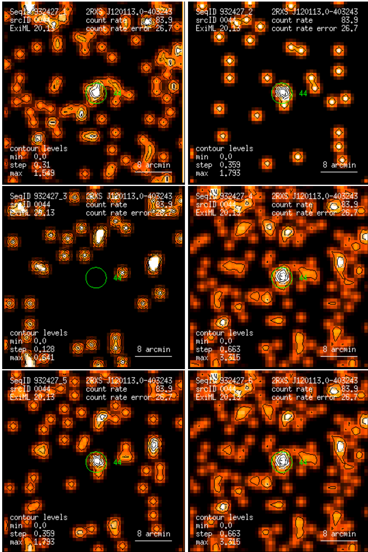
Figure 44: RASS 932427: detection 0044: band rate images, Gaussian filter: (1) PSPC channels 11 – 41, (2) 52 – 90, (3) 91 – 201, (4) 11 – 235, (5) 52 – 201, (6) 11 – 201. Broad band rates in counts/ks. Band rate contour levels in counts/ks/arcmin 2 .
