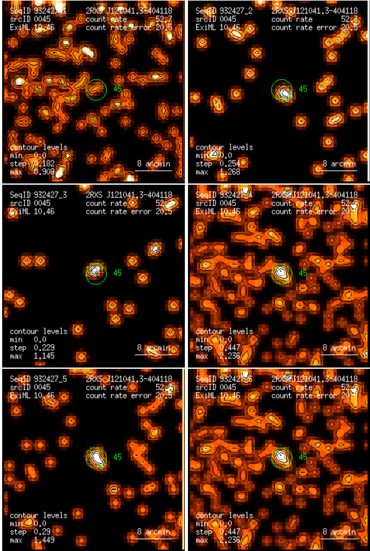
Figure 45: RASS 932427: detection 0045: band rate images, Gaussian filter: (1) PSPC channels 11 – 41, (2) 52 – 90, (3) 91 – 201, (4) 11 – 235, (5) 52 – 201, (6) 11 – 201. Broad band rates in counts/ks. Band rate contour levels in counts/ks/arcmin 2 .
