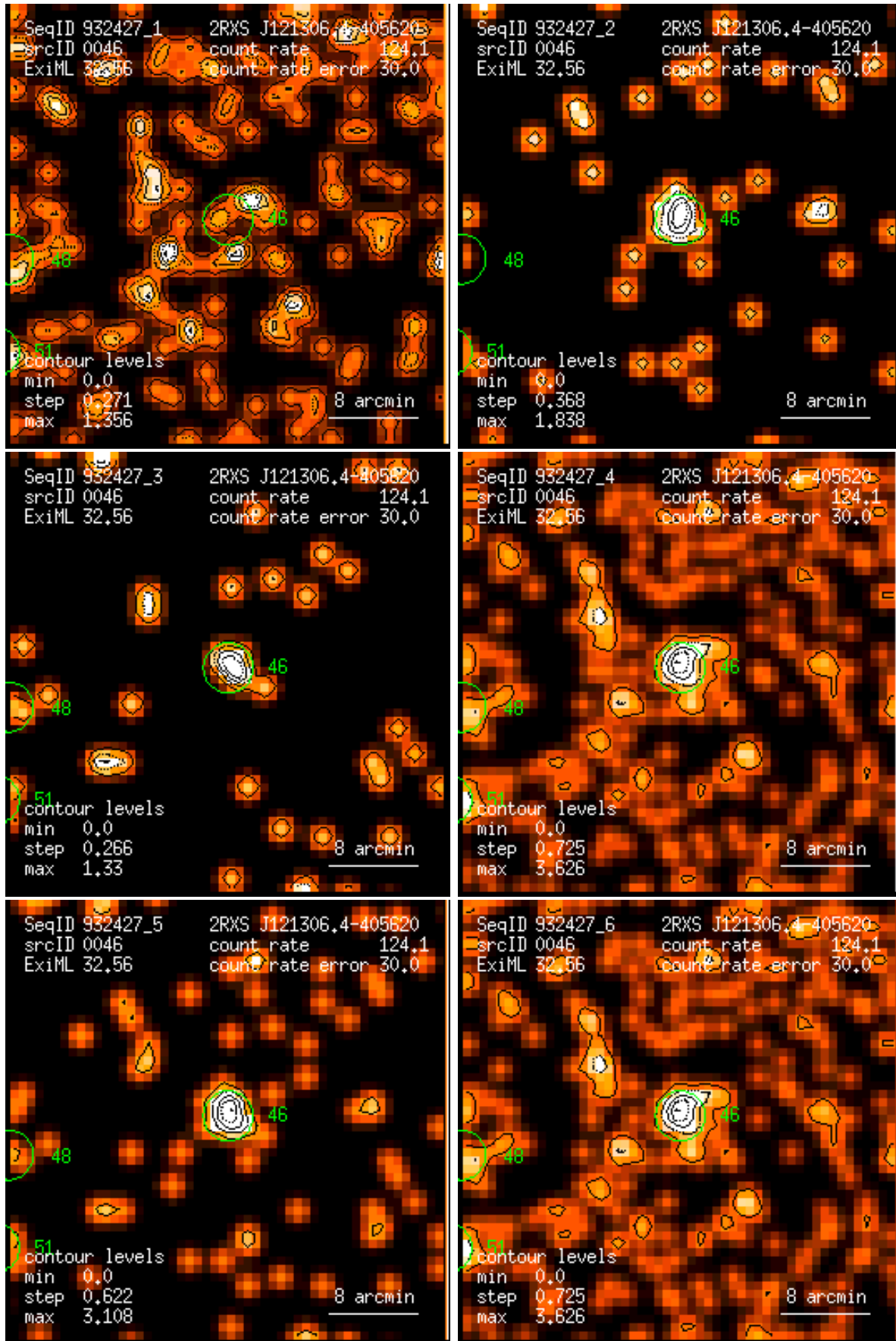
Figure 46: RASS 932427: detection 0046: band rate images, Gaussian filter: (1) PSPC channels 11 – 41, (2) 52 – 90, (3) 91 – 201, (4) 11 – 235, (5) 52 – 201, (6) 11 – 201. Broad band rates in counts/ks. Band rate contour levels in counts/ks/arcmin 2 .
