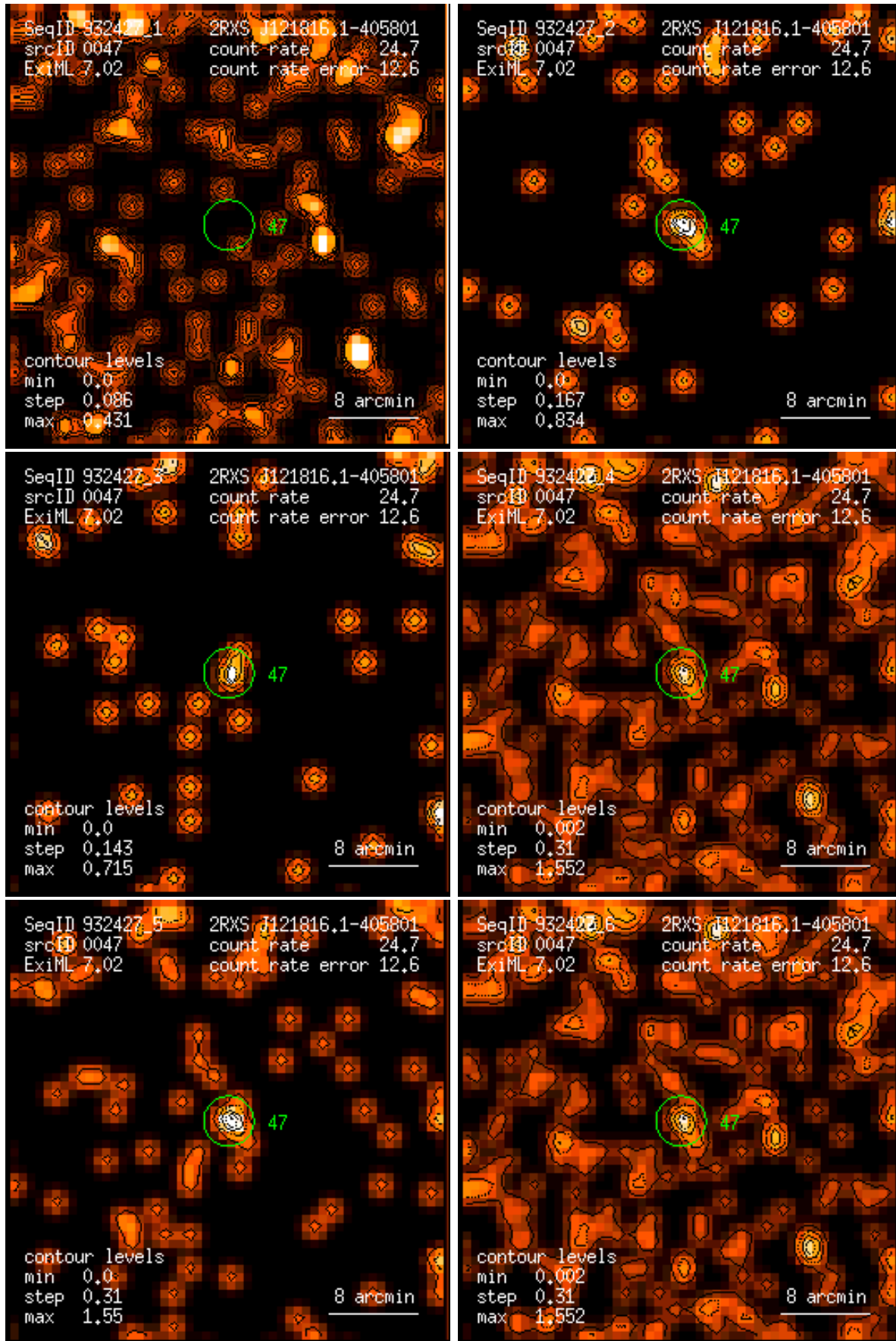
Figure 47: RASS 932427: detection 0047: band rate images, Gaussian filter: (1) PSPC channels 11 – 41, (2) 52 – 90, (3) 91 – 201, (4) 11 – 235, (5) 52 – 201, (6) 11 – 201. Broad band rates in counts/ks. Band rate contour levels in counts/ks/arcmin 2 .
