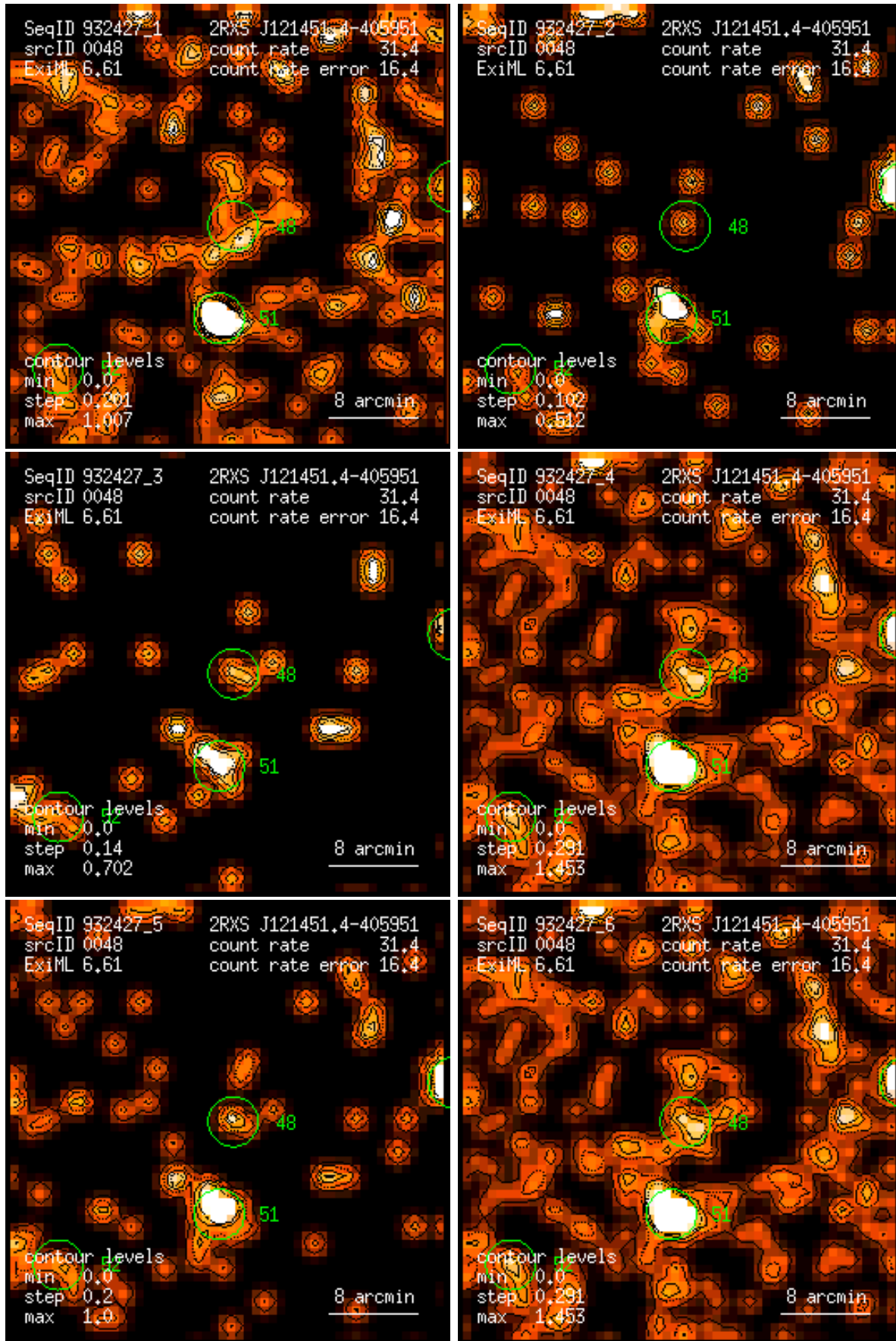
Figure 48: RASS 932427: detection 0048: band rate images, Gaussian filter: (1) PSPC channels 11 – 41, (2) 52 – 90, (3) 91 – 201, (4) 11 – 235, (5) 52 – 201, (6) 11 – 201. Broad band rates in counts/ks. Band rate contour levels in counts/ks/arcmin 2 .
