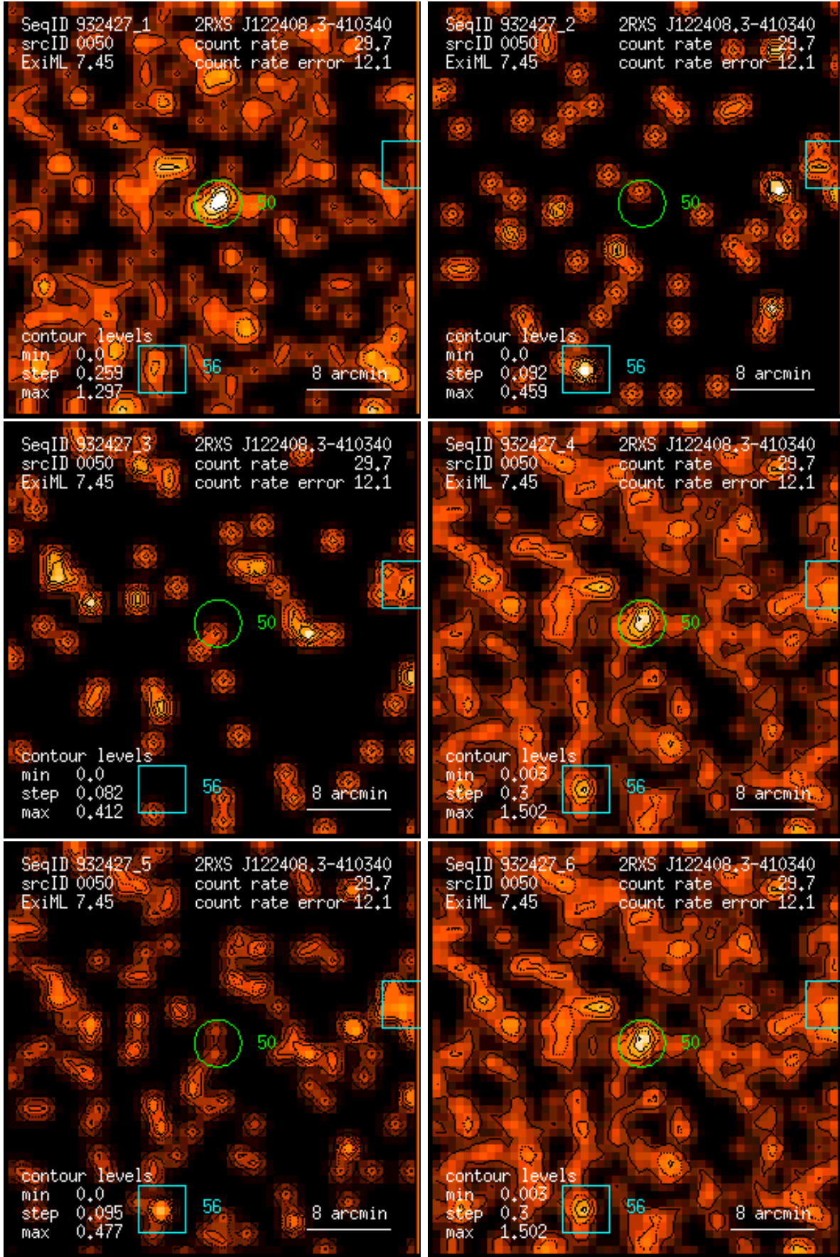
Figure 50: RASS 932427: detection 0050: band rate images, Gaussian filter: (1) PSPC channels 11 – 41, (2) 52 – 90, (3) 91 – 201, (4) 11 – 235, (5) 52 – 201, (6) 11 – 201. Broad band rates in counts/ks. Band rate contour levels in counts/ks/arcmin 2 .
