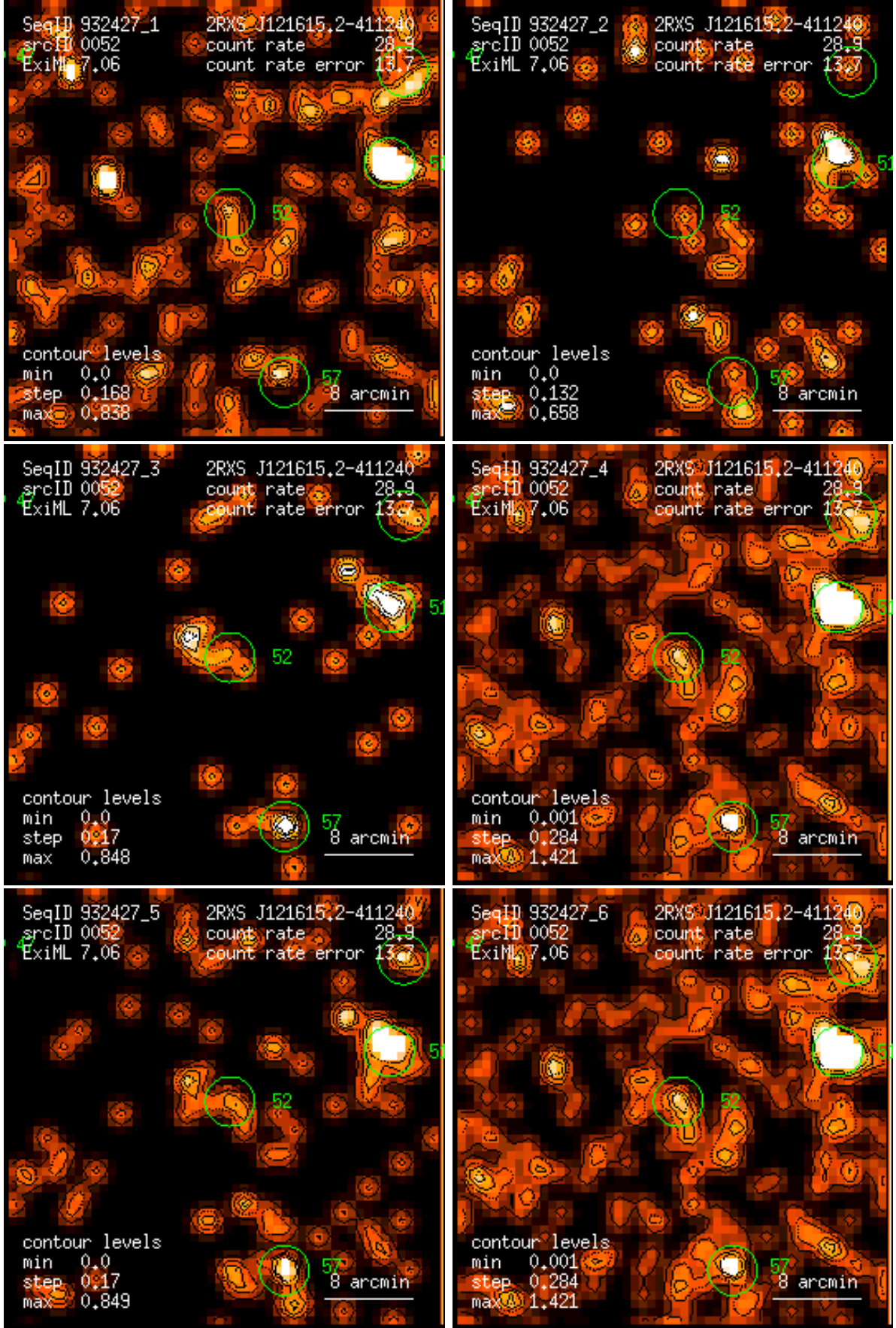
Figure 52: RASS 932427: detection 0052: band rate images, Gaussian filter: (1) PSPC channels 11 – 41, (2) 52 – 90, (3) 91 – 201, (4) 11 – 235, (5) 52 – 201, (6) 11 – 201. Broad band rates in counts/ks. Band rate contour levels in counts/ks/arcmin 2 .
